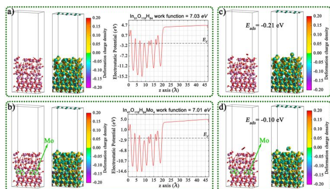
Fig. 8 Geometric structures, charge density difference, calculated work functions, and CO 2 adsorbed on the (001) surface for (a,c) InOOH/In(OH) 3 and (b,d) Mo doped InOOH/In(OH) 3 heterojunction.
