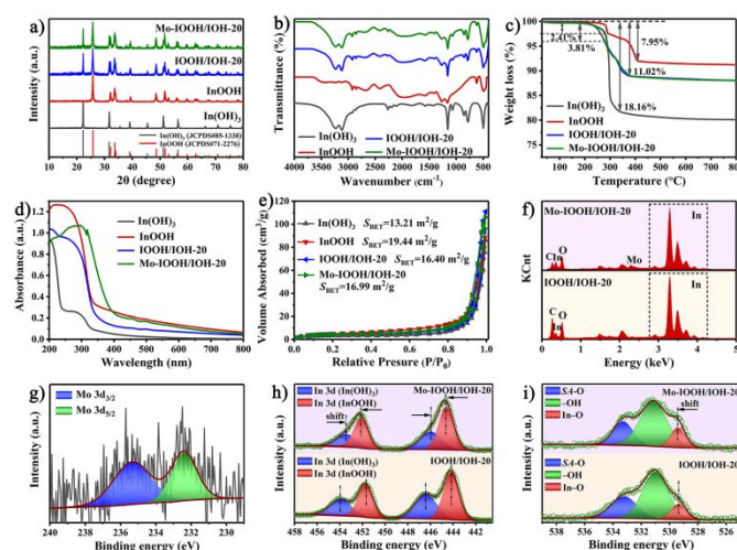
Fig. 2 (a) XRD patterns, (b) FT-IR spectra, (c) TGA curves, (d) UV-vis diffuse reflectance spectra, and (e) N 2 adsorption-desorption isotherms of In(OH) 3 , InOOH, IOOH/IOH-20, and Mo-IOOH/IOH-20. (f) EDS spectra of IOOH/IOH-20 and Mo-IOOH/IOH-20. (g) XPS spectrum for Mo-IOOH/IOH-20 in the region of Mo 3d. (h,i) XPS spectra for IOOH/IOH-20 and Mo-IOOH/IOH-20 in regions of In 3d and O 1s.
