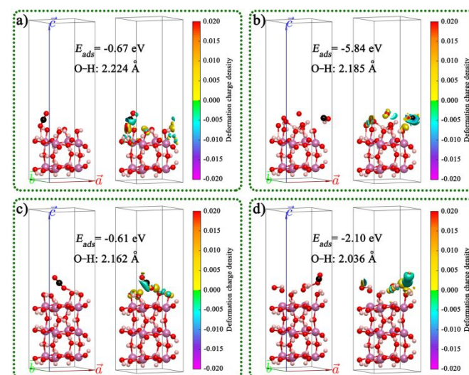
Fig. 7 \text{CO}_2 adsorbed on the (001) surface of \text{In}(\text{OH})_3 with different section thicknesses, exposed atoms, and adsorption sites: (a) \text{In}_8\text{CO}_{26}\text{H}_{24} , (b) \text{In}_8\text{CO}_{30}\text{H}_{28} , (c) \text{In}_{12}\text{CO}_{38}\text{H}_{36} , and (d) \text{In}_{12}\text{CO}_{40}\text{H}_{40} .
