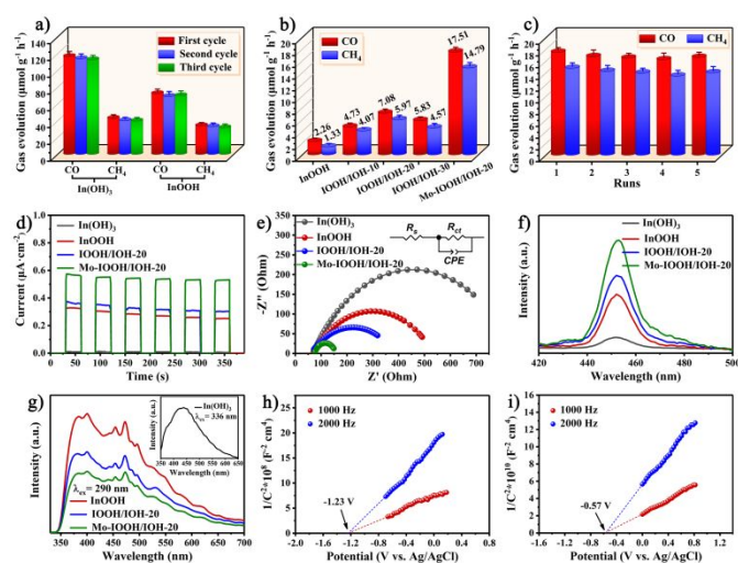
Fig. 3 (a) Production of \text{CO} and \text{CH}_4 for \text{InOOH} and \text{In}(\text{OH})_3 under ultraviolet light irradiation. (b) Production of \text{CO} and \text{CH}_4 for different samples under visible light irradiation. (c) Production of \text{CO} and \text{CH}_4 for \text{Mo-IOOH}/\text{IOH}-20 in five cycles. (d) Photocurrent-time profiles, (e) Nyquist plots with the equivalent circuit as the insert, (f) Fluorescence spectra related to the produced hydroxyl radicals, and (g) PL spectra of different samples. Mott-Schottky plots of (h) \text{In}(\text{OH})_3 and (i) \text{InOOH} .
