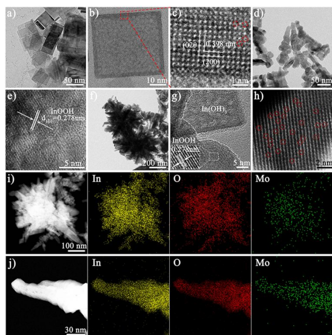
Fig. 1 (a-c) TEM and HRTEM images of In(OH) 3 . (d,e) TEM and HRTEM images of InOOH. (f-h) TEM, HRTEM, and AC HAADF-STEM images of Mo-IOOH/IOH-20. (i,j) The HAADF-STEM image and EDX elemental mappings of Mo-IOOH/IOH-20 with low magnification and high magnification, respectively.
