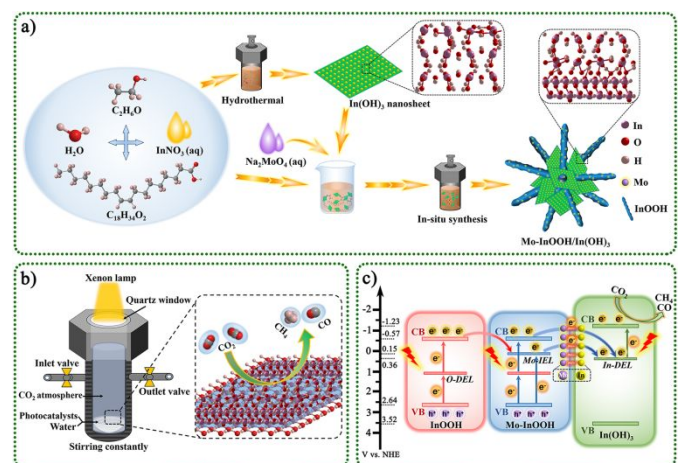
Scheme 1. (a) Synthesis diagrams of Mo modified \text{InOOH}/\text{In}(\text{OH})_3 . (b) Schematic diagram of the \text{CO}_2 photo-reaction system. (c) The proposed mechanism diagram of photocatalysis under visible-light irradiation ( \lambda > 420 nm).
