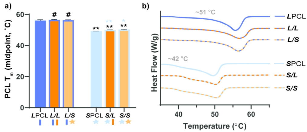
(a) Midpoint T_m of PCL of scaffolds; * p < 0.05 , ** p < 0.01 , # p > 0.05 . Note: The "black color-coded statistics" are comparisons to LPCL and "blue color-coded statistics" are comparisons to SPCL. (b) Representative thermogram for each scaffold composition.
