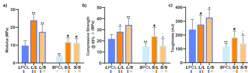
Compressive mechanical properties were compared including (a) E, (b) CS, and (c) toughness; * p < 0.05 , ** p < 0.01 , # p > 0.05 . Note: The "black color-coded statistics" are compared to the LPCL and "light blue color-coded statistics" are compared to SPCL.
