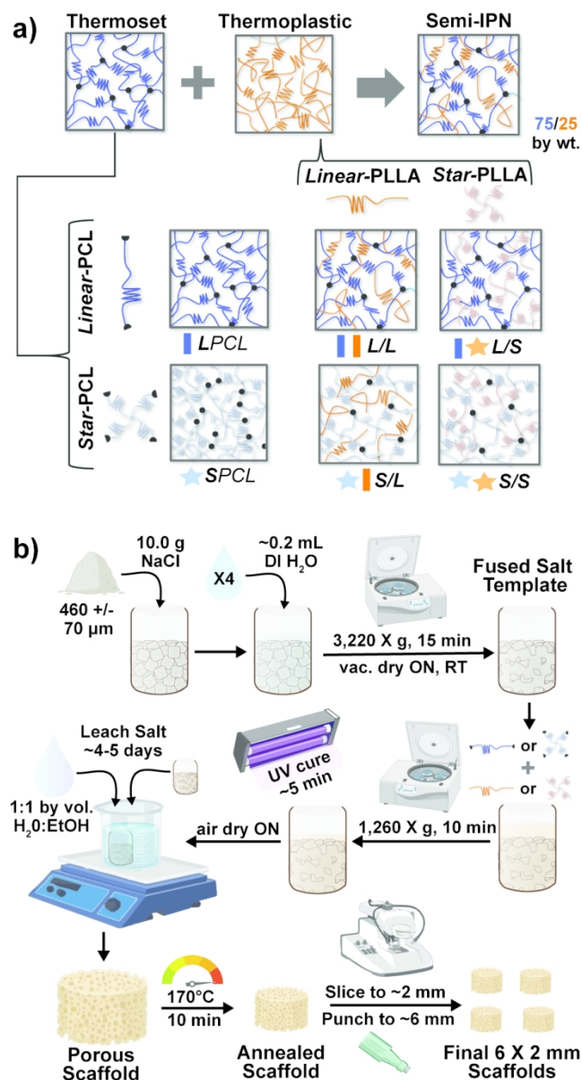
(a) Four semi-IPN SMP scaffolds were prepared with combinations of linear-PCL-DA or star-PCL-TA and linear-PLLA or star-PLLA (75/25 PCL/PLLA). Two 100% PCL controls were also prepared from linear-PCL-DA or star-PCL-TA. (b) All SMP scaffolds were prepared via solvent-casting/particulate leaching (SCPL) whereby a designated solvent-based macromer solution was sequentially cast over a fused salt template, UV-cured, and the template extracted to yield highly interconnected pores.
