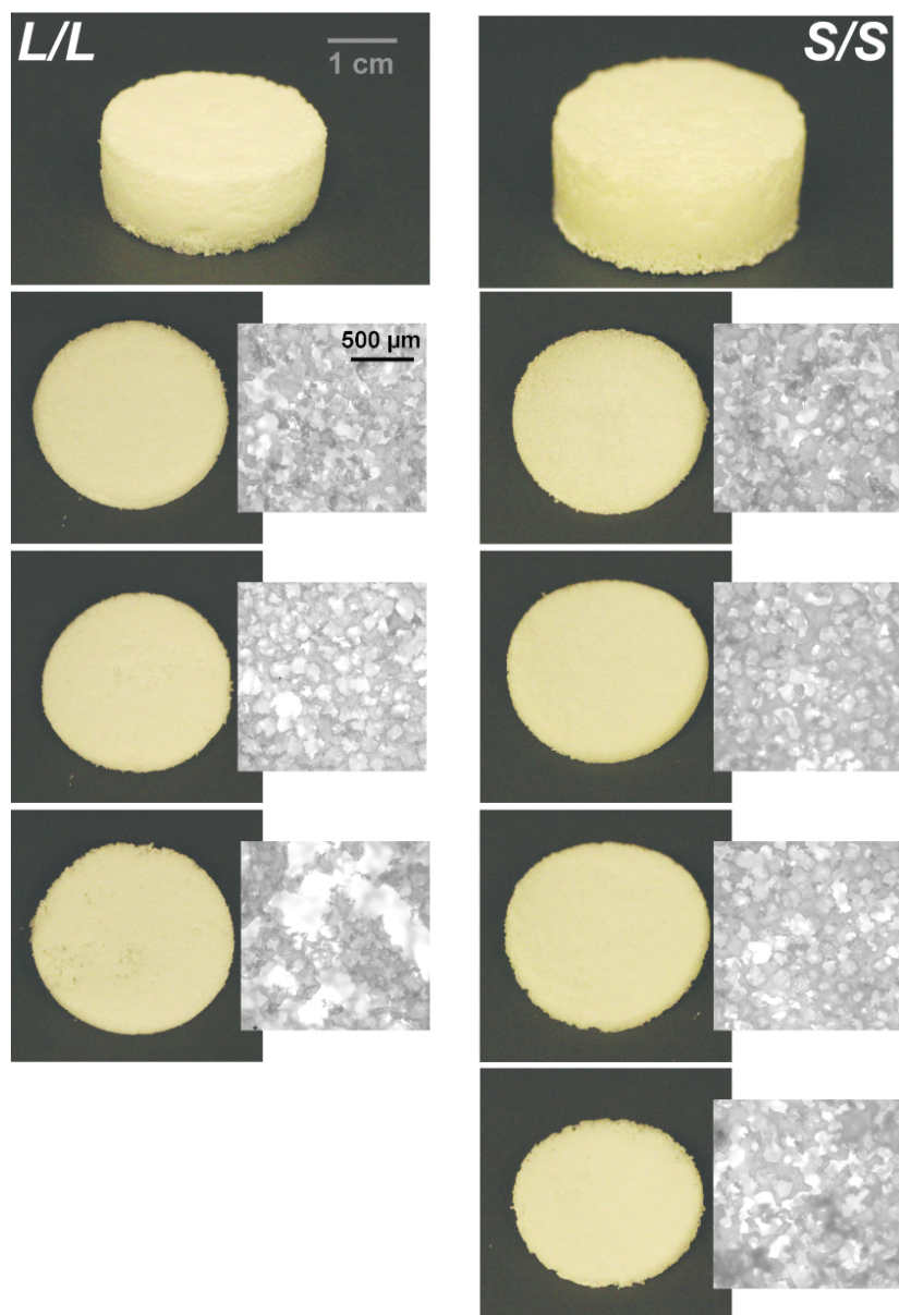
Photos and optical microscopy (5X) of scaled-up, "large" L/L and S/S scaffolds ( d \sim 24 mm) demonstrating superior macromer diffusion, and more uniform pores, for the S/S composition.
