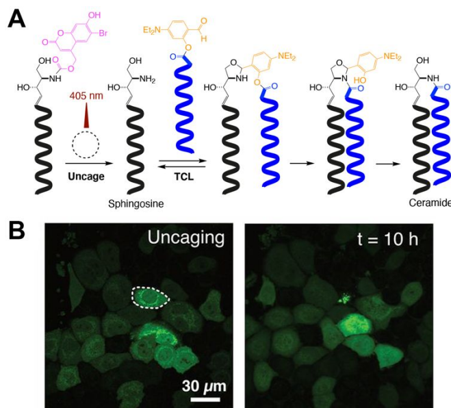
Fig 3 Photocontrolled traceless ceramide ligation (TCL). 11 (A) Photocaged sphingosine is irradiated with 405 nm laser light to produce sphingosine and subsequently trigger TCL with a fatty acid salicylaldehyde ester, which affords the corresponding ceramide. (B) Cellular apoptosis mediated by spatiotemporally controlled TCL. One specific GFP-marked HeLa cell was exposed to 10 s of 405 nm light ( left ), observing its cell death after 10 h of incubation ( right ) [Adapted with permission from A. K. Rudd and N. K. Devaraj, Proc. Natl. Acad. Sci. U. S. A. , 2018, 115 , 7485–7490]. 11
