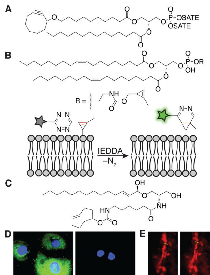
Fig 4 Synthetic lipids for fluorescent, live-cell imaging of lipids. (A) The chemical structure of the cyclooctyne-PA mimic for fluorescent imaging in live cells. 15 (B) A phospholipid with a methyl cyclopropene headgroup enables live-cell imaging after IEDDA tagging with a tetrazine fluorophore. 16 (C) The chemical structure of the trans -cyclooctene-ceramide conjugate for superresolution imaging of the Golgi. 17 (D) Fluorescence microscopy after labeling with probes described in (B). Fluorescence is only observed in the presence ( left ) and not the absence ( right ) of the cyclopropene phospholipid [Adapted from ref. 16 with permission from John Wiley & Sons, copyright 2012]. 16 (E) Confocal ( left ) and stimulated emission depletion superresolution (STED) ( right ) microscopy imaging of the Golgi complex enabled by a trans -cyclooctene-containing ceramide and IEDDA tagging [Adapted from ref. 17 with permission from John Wiley & Sons, copyright 2014]. 17
