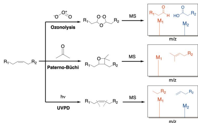
Fig 10 Common strategies for the derivatization of double bonds. The lipid is either treated online or offline, and the double bonds undergo chemical reactions that create distinct fragments, which are then detected in the spectrometer. 46–50
