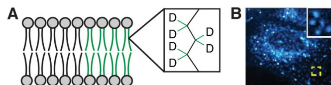
Fig 6 SRS lipid imaging. (A) Deuterated palmitate and oleate incorporated into lipid acyl chains. (B) SRS imaging of C–D single bond stretches in cells treated with palmitate- d_{31} reveals patches of slow lateral diffusion in the ER [Adapted with permission from Y. Shen, Z. Zhao, L. Zhang, L. Shi, S. Shahrir, R. B. Chan, G. Di Paolo and W. Min, Proc. Natl. Acad. Sci. , 2017, 114 , 13394–13399]. 26
