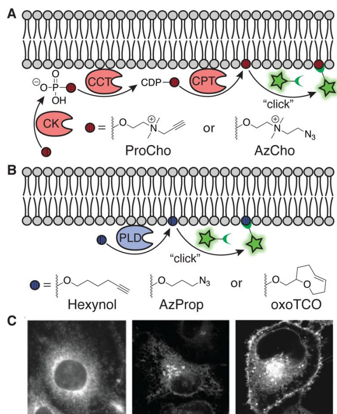
Fig 5 Enzymatic labeling of specific lipid classes. (A) Analogs of choline, ProCho and AzCho, are incorporated via the Kennedy pathway of PC biosynthesis [CK: choline kinase, CCT: phosphocholine cytidylyltransferase, CPT: cholinephosphotransferase]. CuAAC, SPAAC, or Staudinger ligation of the tagged lipids enable fluorescent imaging. 22 (B) IMPACT labeling with non-natural primary alcohols report on phospholipase D (PLD) activity. Fluorophore conjugation via CuAAC, SPAAC, or IEDDA labels pools of PA generated by PLD. (C) Fluorescence imaging of membranes using ProCho after CuAAC tagging (left) [Adapted with permission from C. Y. Jao, M. Roth, R. Welti and A. Salic, Proc. Natl. Acad. Sci. U. S. A. , 2009, 106 , 15332–15337], 18 and localization of PLD activity via IMPACT with AzProp and SPAAC (middle) [Adapted with permission from https://pubs.acs.org/doi/10.1021/acscentsci.7b00222 . Further permissions for the material excerpted should be directed to the American Chemical Society], 21 and RT-IMPACT with oxoTCO after IEDDA tagging (right) [Adapted with permission from D. Liang, K. Wu, R. Tei, T. W. Bumpus, J. Ye and J. M. Baskin, Proc. Natl. Acad. Sci. , 2019, 116 , 15453–15462]. 23
