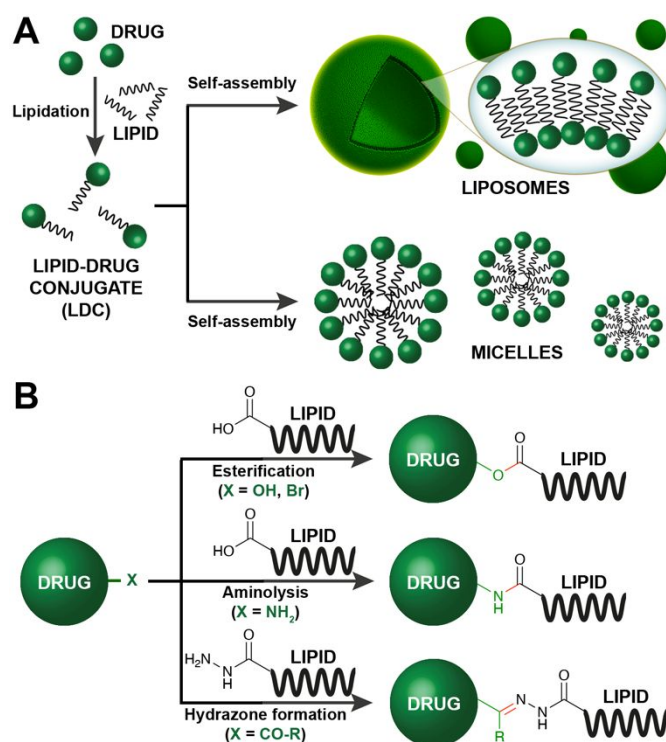
Fig 8 Lipid modification for the construction of enhanced drug carriers. 35-40 (A) Schematic representation of the preparation of drug delivery systems based on the lipidation of the corresponding drug. The drug is initially lipidated, affording a lipid-drug conjugate (LDC), which can spontaneously self-assemble into different type of structures, including liposomes and micelles. (B) Common strategies employed for the formation of LDCs.
