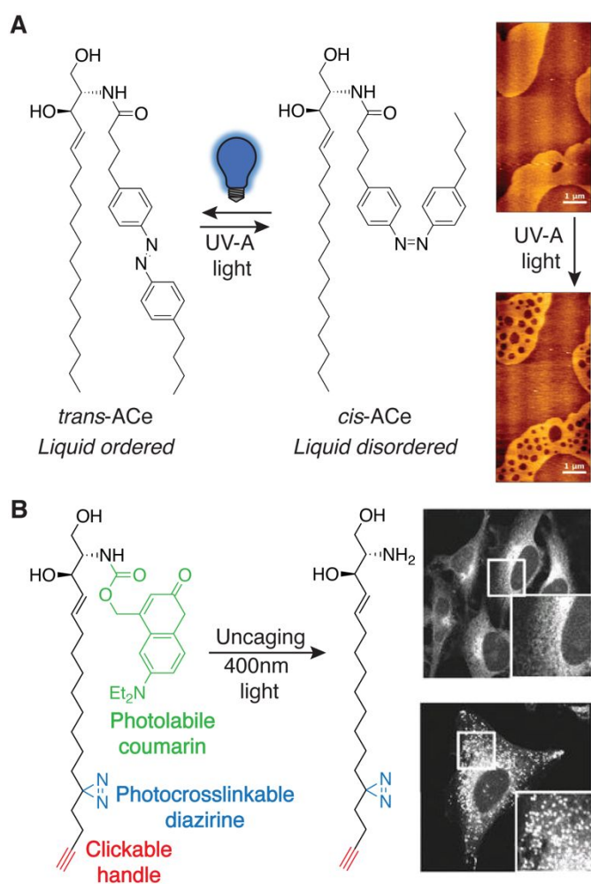
Fig 9 Photoswitchable lipids. (A) Azobenzene-bearing ceramides (ACes) that induce liquid-ordered ( L_o ) membranes as the trans isomer are converted to the liquid-disordered-favoring ( L_d ) cis isomer with UV-A light (365 nm), demonstrated by AFM imaging of ACe containing supported lipid bilayers ( right ) [Adapted with permission from J. A. Frank, H. G. Franquelim, P. Schuille and D. Trauner, J. Am. Chem. Soc. , 2016, 138, 12981–12986. Copyright 2016 American Chemical Society]. 42 (B) A trifunctional sphingosine is selectively uncaged with 400 nm light revealing sphingosine localization with fluorescence imaging in control cells ( top ) and cells where the Niemann-Pick C1 protein (NPC1) was depleted using siRNA ( bottom ), following photocrosslink-mediated immobilization and CuAAC tagging of the sphingosine probe [Adapted with permission from D. Höglinger, A. Nadler, P. Haberkant, J. Kirkpatrick, M. Schifferer, F. Stein, S. Hauke, F. D. Porter and C. Schultz, Proc. Natl. Acad. Sci. U. S. A. , 2017, 114 , 1566–1571]. 44
