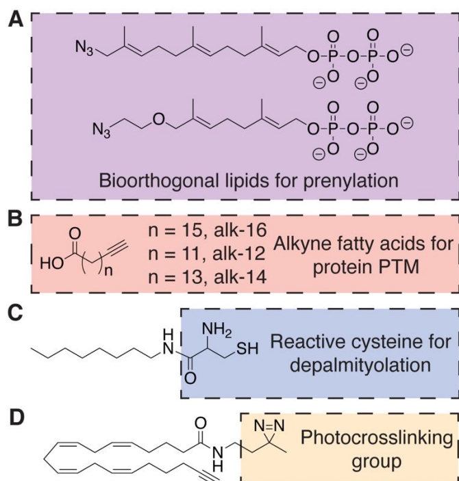
Fig 7 Chemical structures of probes for the posttranslational lipidation of proteins. 27–31 (A) Azido isoprenoids identify sites of prenylation in the proteome. (B) Fatty acids with terminal alkynes to study protein lipidation. (C) A substrate for amphiphile-mediated depalmitoylation (AMD) native chemical ligation. (D) Example of a bifunctional lipid containing a photocrosslinkable diazirine functional group and terminal alkyne.
