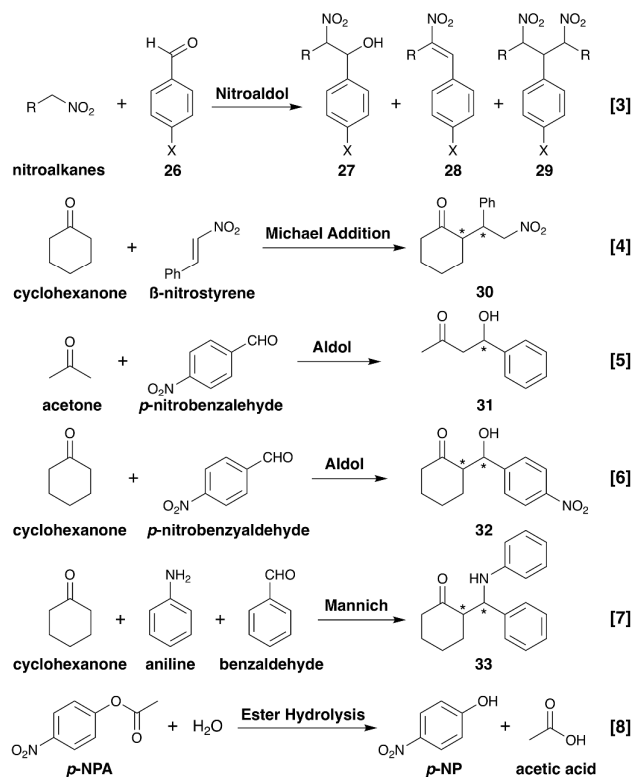
Scheme 4. Various standard chemical transformations known to be catalyzed by self-assembled peptide catalysts.
