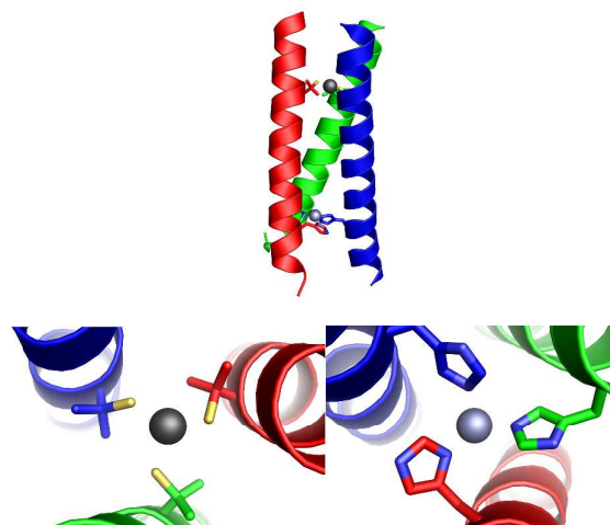
Figure 6. (Top) X-ray crystal structure (PDB 3PBJ) of an artificial metalloenzyme [\text{Hg(II)}]_5[\text{Zn(II)(OH}^-)]_N(\text{TRIL9CL23H})_3 with multiple metal-binding sites. (Bottom left) Binding of thiolates to Hg(II) provides stability to metalloenzyme. (Bottom right) The catalytic zinc site.
