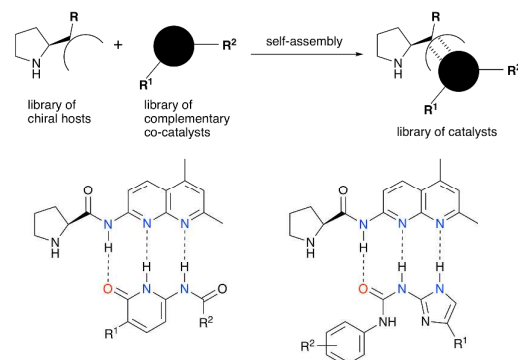
Scheme 1. Self-assembly of Pro-Nap with co-catalysts. Reproduced from ref. 51 with permission from the Royal Society of Chemistry, copyright 2011.
