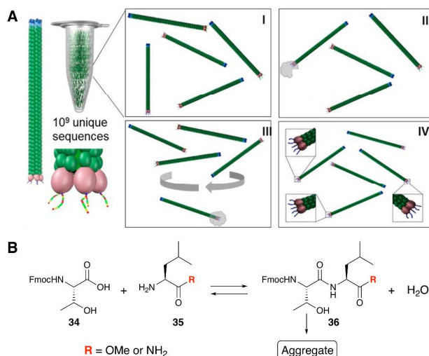
Figure 21. Illustration of screening phage libraries for catalytic activity. (A) Four cycles of phage replication were necessary to generate an expansive library of sequences. (B) Dipeptides formed by condensation of Fmoc-Thr with leucine derivatives aggregate driving the equilibrium to the right. Reproduced from ref. 124 with permission from the American Chemical Society, copyright 2014.
