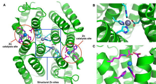
Figure 13. (A) A crystal structure of the catalytically active artificial hydrolase, \text{Zn}_8:\text{AB}_3_4 (PDB 3IQ6). Two types of sites – structural and catalytic – are indicated (only half of the bundle is shown for clarity). (B) Enhanced view of the structural zinc coordination sphere. (C) Enhanced view of the catalytic zinc coordination sphere.
