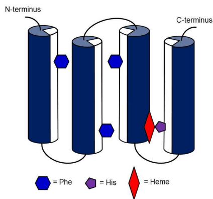
Figure 10. Schematic representation of secondary elements of C45: His to Phe mutations help to stabilize the desired structure and direct heme binding to a histidine.
