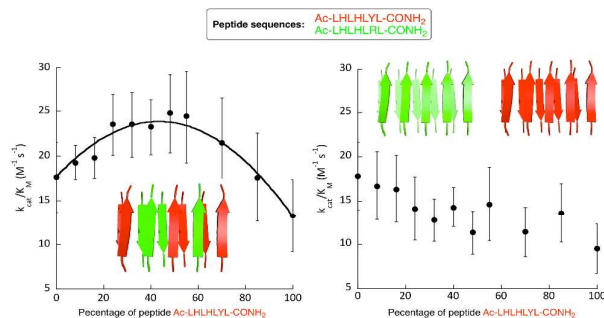
Figure 23. Illustration of synergistic effect in catalytic amyloids. Fibrils formed from a mixture of peptides (left) show higher activity than homomeric peptide mixtures (right). Reproduced from ref. 133 with permission from Nature Publishing Group, copyright 2014.
