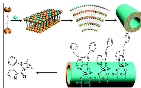
Scheme 5. Formation of catalyst by self-assembly of monomers into multi-layered nanotubes (blue cylinders) in the presence of Cu(II) (blue spheres). Reproduced with permission from ref. 131. Reproduced from ref. 131 with permission from the American Chemical Society, copyright 2011.
