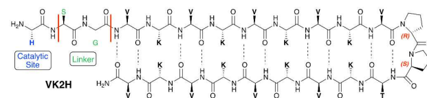
Figure 20. Self-assembling peptide VK2H formed by attaching a catalytic His (blue) to MAX1 with a Ser-Gly linker (green).
