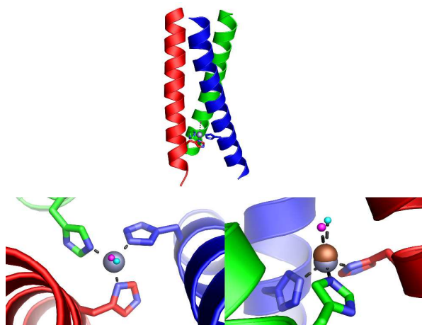
Figure 8. (Top) The model of the peptide \text{Cu(I/II)}(\text{TRIL23H})_3 based on a crystal structure of a related protein [\text{Hg(II)}]_5[\text{Zn(II)(OH)}]_n(\text{TRIL9CL23H})_3 (PDB code 3PBJ). (Bottom left) Top-down perspective of the metal binding site in metalloprotein. (Bottom right) Comparison of the metal binding sites with Zn (gray) and Cu (brown). Water molecules from two different structures are shown as magenta and cyan spheres.
