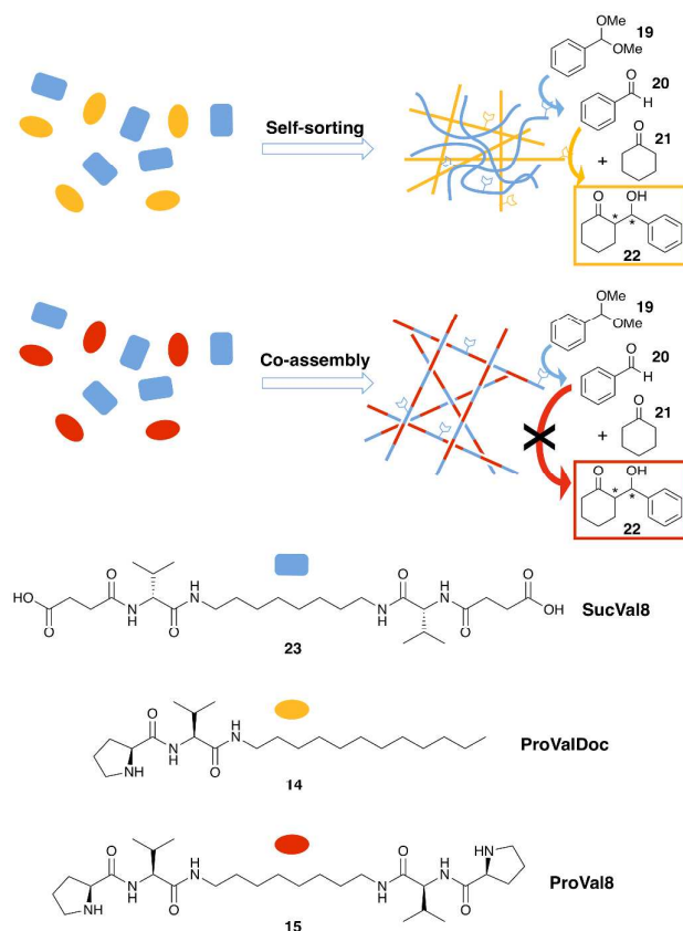
Scheme 3. Self-sorting versus co-assembly in tandem deacetalization/aldol coupling reaction. Randomly assorted fibrils that “self-sort” facilitate conversion of the acetal to the aryl aldehyde and its subsequent aldol coupling with cyclohexanone. Co-assembled fibrils do not promote aldol coupling. Reproduced from ref. 105 with permission from the Royal Society of Chemistry, copyright 2016.
