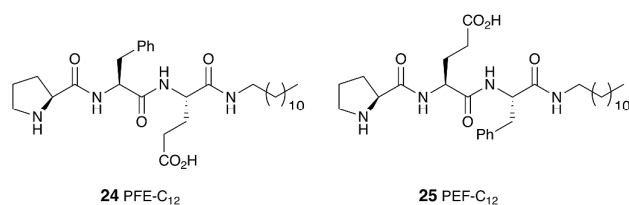
Figure 16. Pro-Phe-Glu-based catalysts capable of aldol reaction catalysis.
