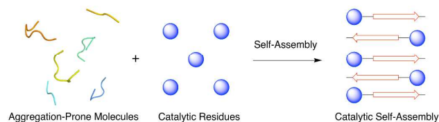
Scheme 2. Overall approach to creating self-assembling peptide catalysts.
