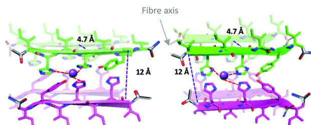
Figure 25. Proposed structure based on X-RFD data for the peptide assemblies formed by Ac-IHIHIYI-CONH 2 . Reproduced from ref. 138 with permission from the Royal Society of Chemistry, copyright 2017.
