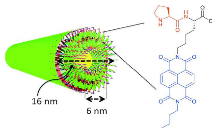
Figure 17. A model for catalytic nanotubes formed by Pro-Lys-NDI. Adapted from ref. 110 with permission from the Royal Society of Chemistry, copyright 2015.
