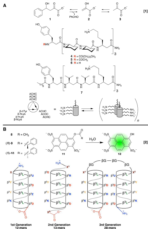
Figure 14. (A) Retroaldol-catalyzed reaction of 1 by catalytic assemblies 4-6 derived from ACHC-scaffold or assembly 7 . A helical-wheel diagram of the \beta -peptide (left) and cartoon representation of the assembly (right) are shown. (B) Helical diagrams of \beta^3 -peptide assemblies (1 st , 2 nd , and 3 rd generations) tested in the hydrolysis of pyrene trisulfonate esters. Reproduced from ref. 84 and 86 with permission from Wiley-VCH Verlag GmbH & Co. KGaA (copyright 2008) and from the American Chemical Society, (copyright 2014).
