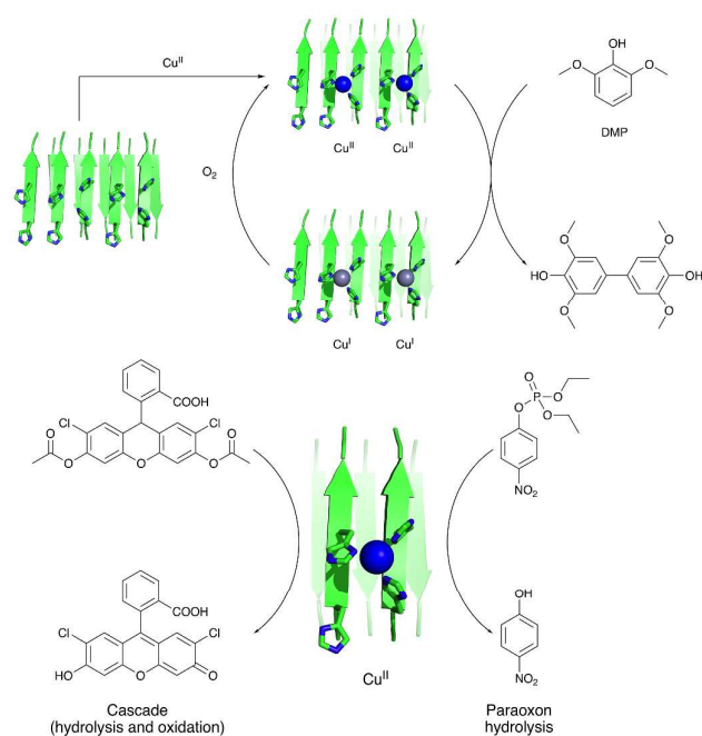
Scheme 6. Representative model of copper-binding catalytic amyloids capable of catalyzing oxidative (top), hydrolytic (bottom right) and cascade (bottom left) reactions. Reproduced from ref. 136 and ref. 140 with permission from the American Chemical Society (copyright 2017) and from Wiley-VCH Verlag GmbH & Co. KGaA (copyright 2016).
