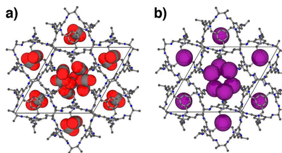
Figure 4. Crystal structures of a) CC2 •6CO 2 and b) Xe in CC2 determined from in situ PXRD data. Cages are shown as ball and stick models (hydrogen atoms omitted) and guests as space-filling representations using van der Waals radii.
