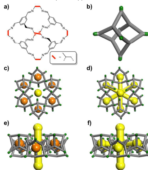
Figure 1. a) Chemical structure of the porous cage, CC2 ; b) Simplified 3D representation of the CC2 cage where vertices are coloured green. CC2 forms window-to-arene stacks and the methyl vertices frustrate packing to give 1D inter-stack pore channels (yellow); the crystal structure also displays voids (orange), which encircle these 1-D channels as shown both c) down the channels and; e) orthogonal to the channels. Static porosity analysis, treating the molecules as rigid and immobile, shows that the voids and the 1D channels are disconnected (c, e). By contrast, dynamic and cooperative porosity analyses suggest that the cage voids can be linked to the channels, d) and f), but that the degree of linking is guest dependent.
