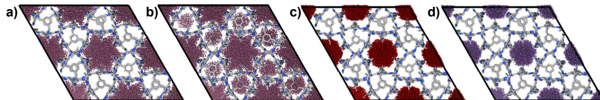
Figure 3. The empty host MD simulations were analysed using Zeo++ to highlight the accessible void volume determined for the guest-free CC2 crystal structure. Superimposition of the H 2 -accessible void volume for a) two artificially methyl-ordered models versus, b) the methyl-disordered CC2 models. Comparison of a) and b) shows how the relative positions of the methyl groups affect the guest accessibility of the cage cavities. The accessible void volume for c) CO 2 , and d) Xe for all 10 superimposed models; these simulations suggest that diffusion from channel to cage would not be observed for these large guests on the MD timescale, irrespective of the relative methyl group positions. The radii used were H 2 = 1.09 Å, CO 2 = 3.40 Å, Xe = 2.05 Å.
