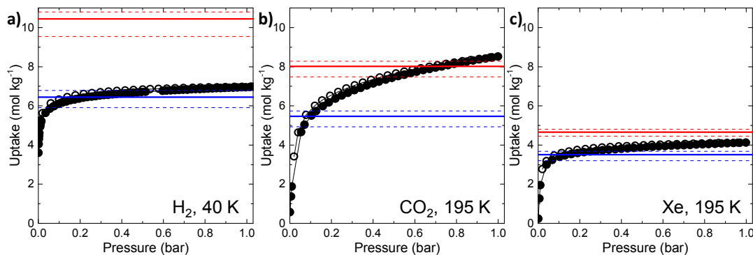
Figure 2. Simulated and experimental gas sorption results for CC2 for (a) \text{H}_2 , (b) \text{CO}_2 , and (c) Xe. Experimental measurements are represented as black, filled circles (adsorption) and empty circles (desorption). Simulated uptakes at 1 bar are given as red lines (all sites accessible) and blue lines (intrinsic cage cavities blocked): the solid lines represent the average values of the 10 models, while the dashed lines indicate the maximum and minimum values in the set, respectively.
