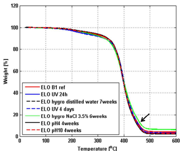
Figure 4 Thermogravimetric analysis (TGA) data showing weight loss of specimens as a function of temperature between 25°C and 600°C. Note that there is no peak corresponding to water evaporation present and that the only difference in behaviour is observed for sample that has undergone hygrothermal ageing in NaCl solution (green line).
