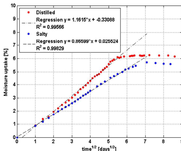
Figure 2 Gravimetric analysis of a hygrothermally aged resin sample (40°C; distilled water – red and 3.5% NaCl – blue). The dashed lines represent linear regression fit to the first 28 data points.
