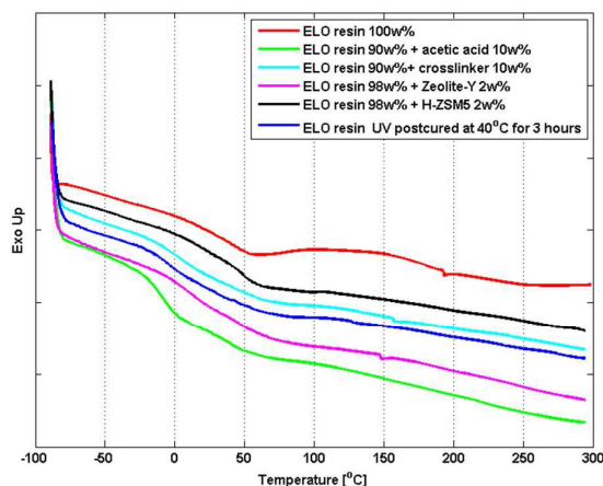
Figure 14 Differential Scanning Calorimetry (DSC) data showing heat flux as a function of temperature between -90^{\circ}\text{C} and 300^{\circ}\text{C} . Data for each series has been offset along the vertical axis to highlight the differences and similarities between particular samples.
