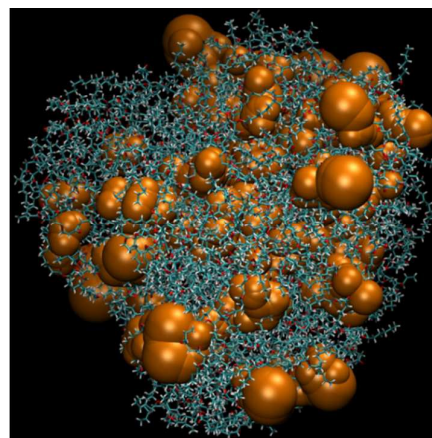
Figure 9 Snapshot of the ELO resin model from MD simulations (GAFF 31,32 force field, temperature 340K, simulation time: 100ns) in vacuum. Cavities that could accommodate water have been highlighted as orange surfaces.
