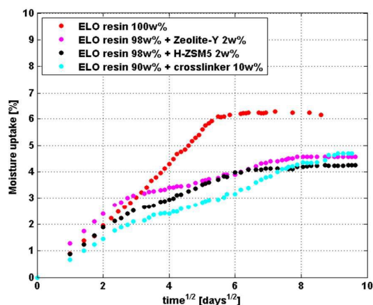
Figure 15 Gravimetric analysis of a hygrothermally aged ( 40^{\circ}\text{C} ; distilled water) resin samples with and without the additives showing the positive influence of the additives on resins water resistance
