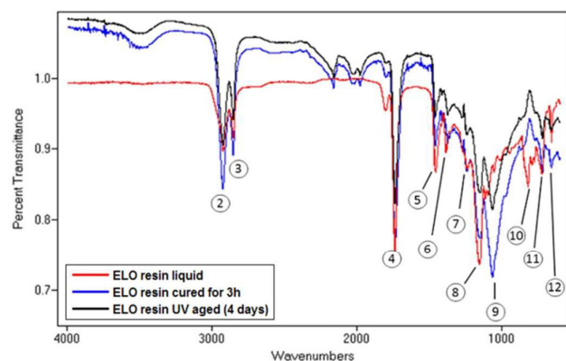
Figure 5 Comparison of the FT-IR spectra of liquid resin (red), the solid sample that was cured for 3 hours (blue) and solid sample that has been post-cured for additional 4 days (black). Note the partial disappearance of the peaks corresponding to the oxirane rings and the emergence of the ether bridge signature following the curing process (see also Table 1 for chemical assignments).
