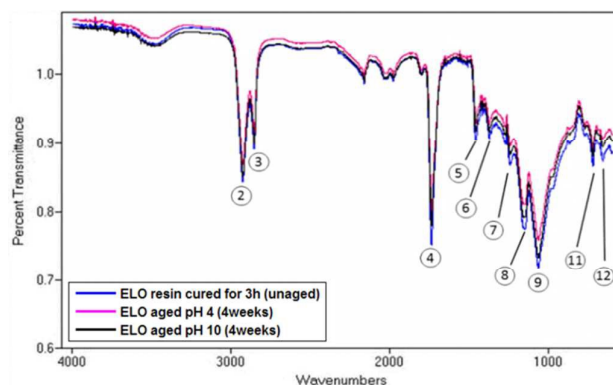
Figure 6 Comparison of the FT-IR spectra of the UV-cured (3h) solid resin (blue line) and its corresponding analogues that were subjected to strongly acidic environment (pH 4) (magenta line) and strongly basic environment (pH 10) for 4 weeks (black line).
