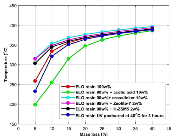
Figure 13b TGA data showing the mass-loss temperature versus mass-loss for ELO resin with different additives.
