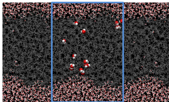
Figure 11 Snapshot from the periodic MD simulations of the ELO monomers in water, showing water permeation into a periodic slab of ELO. Water molecules that have permeated into the bulk ELO are highlighted. The periodic cell is highlighted with a blue box, but for formatting purposes the image has been truncated in the vertical axis. A non-truncated version of this Figure is available in the supplementary information (Figure S4).
