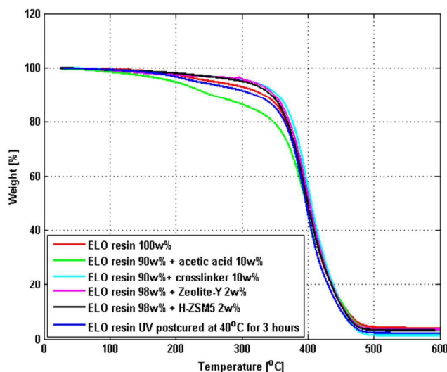
Figure 13a Thermogravimetric analysis (TGA) data showing weight loss of the specimens as a function of temperature between 25^\circ\text{C} and 600^\circ\text{C} . Note that a significant difference in behaviour is observed for samples altered by the addition of acetic acid and also with ZSM-5 and Zeolite Y.
