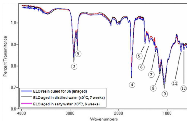
Figure 7 Comparison of the FT-IR spectra of the UV-cured (3h) solid resin (blue line) and its corresponding analogues that were subjected to hygrothermal treatment at 40°C in distilled (black line) and salty (3.5% NaCl) water (magenta line) for 7 and 6 weeks respectively. Note the highlighted reduction in the intensity of the 12th peak (O-H out of plane bend alcohol).
