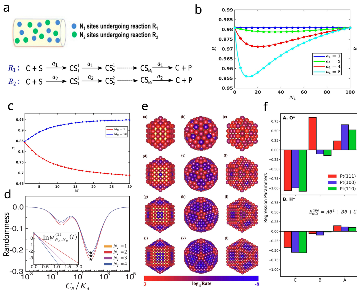
Fig. 6 Schematic representation of a nanoparticle catalyst with two different types of, N_1 and N_2 , catalytically active sites. (bottom) The chemical reaction taking place on each type of site. Randomness parameter as a function of (b) N_1 while keeping N_2 constant, (c) M_1 while keeping M_2 constant. (d) Randomness for heterogeneous model with substrate concentration. (e) CO oxidation rates schematic on surface sites of Au clusters of different geometry. (f) Fitted parameters A, B, and C, for the adsorption energies model for O and H. Figures (a,b,c) Reproduced from ref 97 , with the permission of AIP Publishing. Figure (d) reproduced with permission from ref 145 . Copyright 2021 American Physical Society. Figure (e) reproduced with permission from ref. 146 . Copyright 2018 American Chemical Society. Figure (f) reproduced with permission from ref 34 . Copyright 2024 American Chemical Society.
