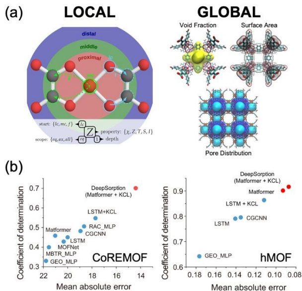
Figure 2. (a) Examples of local and global features. The depicted local feature is the revised autocorrelation (RAC for start_z scope_z depth ) function that quantifies the discrete correlation of Z (electronegativity, nuclear charge, topology, covalent atomic radius, and identity for \chi, Z, T, S , and I , respectively) between atoms separated up to depth l . The start index (ligand-centered, metal-centered, and full for lc, mc , and f , respectively) refers to the reference of the RAC summation and the scope index (axial, equatorial, and all for ax, eq , and all , respectively) refers to which neighboring ligand atoms are included in the summation. Reprinted with permission from ref 24 . Copyright 2017, American Chemical Society. The depicted global features show commonly used geometric descriptors. Adapted with permission from ref 25 . Copyright 2020, American Chemical Society. (b) Comparison of machine learning model performance using different architectures and features for CO 2 adsorption using the (left) CoREMOF and (right) hMOF datasets. In general, increasingly complex models (from MLPs trained on geometric features (GEO_MLP) to transformers trained on chemical and positional encodings (Matformer)) that learn “long-range” spatial correlations between local features tend to improve model performance. Adapted from ref 26 .
