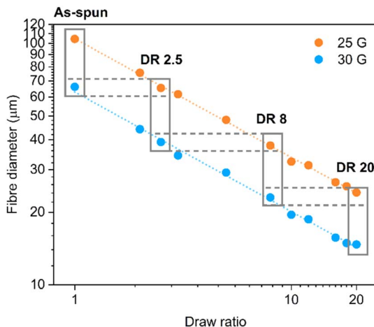
Fig. 3 Relationship between fibre diameter and ratio (DR) for lignin–PVA fibres extruded through 25 G (260 \mu\text{m} ) and 30 G (159 \mu\text{m} ) spinnerets. Vertically oriented boxes indicate fibres with the same draw ratio (but different diameter) and horizontally oriented boxes (dashed) indicate hot-drawn fibres with the same diameter (but different draw ratios). The orange and blue lines (dotted) fitted to the 25 G and 30 G data have slopes of -0.49 and -0.50 , respectively.
