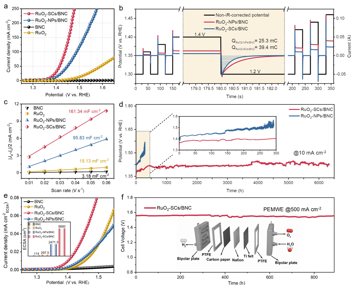
Fig. 4 Electro-catalytic acidic OER performance. (a) LSVs of RuO 2 , BNC, RuO 2 -NPs/BNC and RuO 2 -SCs/BNC conducted at a 5 mV s -1 scan rate, in a 0.5 M H 2 SO 4 solution with iR correction. (b) Pulse voltammetry protocol curves of RuO 2 -NPs/BNC and RuO 2 -SCs/BNC. (c) C dl plots of RuO 2 , BNC, RuO 2 -NPs/BNC and RuO 2 -SCs/BNC. (d) Chronopotentiometry test for RuO 2 -NPs/BNC and RuO 2 -SCs/BNC at 10 mA cm -2 . The inset shows a magnified plot of stability in the first 300 hours. (e) ECSA-normalized OER activity of BNC, RuO 2 , RuO 2 -SCs/BNC and RuO 2 -NPs/BNC. The inset shows the detailed ECSA values. (f) PEM device performance (500 mA cm -2 ) using commercial Pt/C and RuO 2 -NPs/BNC as catalysts in the PEM electrolyzer. A schematic of the PEM electrolyzer is shown in the inset, in which the anode and cathode sides are separated by a Nafion membrane.
