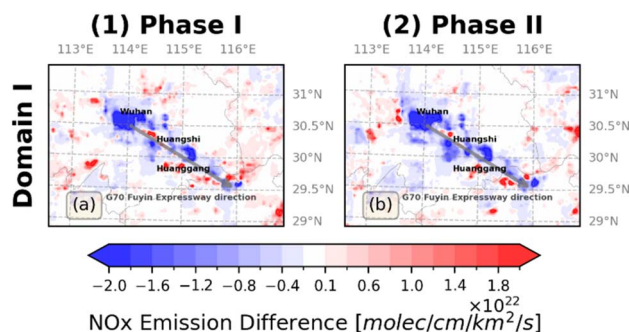
Fig. 6 High-resolution NO x emission changes across study domains during COVID-19 lockdown phases relative to pre-lockdown baseline. Spatial distribution of NO x emission differences ( \times 10^{22} molecules \text{cm}^{-2} \text{km}^{-2} \text{s}^{-1} ) for (a) Phase I (lockdown period, left column) and (b) Phase II (recovery period, right column) compared to pre-lockdown levels for Domain I (Hubei Area). Blue colors indicate emission decreases while red colors represent emission increases relative to baseline conditions. Major cities are labeled within each domain.
