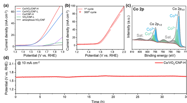
Fig. 4 (a) Polarization curves of Co/VO_x/CNF-H , Co/VO_x/CNF-L , VO_x/CNF-L , and amorphous VO_x/CNF . (b) Polarization curves of Co/VO_x/CNF-H before and after 300 CV cycles. (c) XPS Co 2p spectra of Co/VO_x/CNF-H after 300 CV cycles. (d) Chronopotentiometry curve of Co/VO_x/CNF-H .
