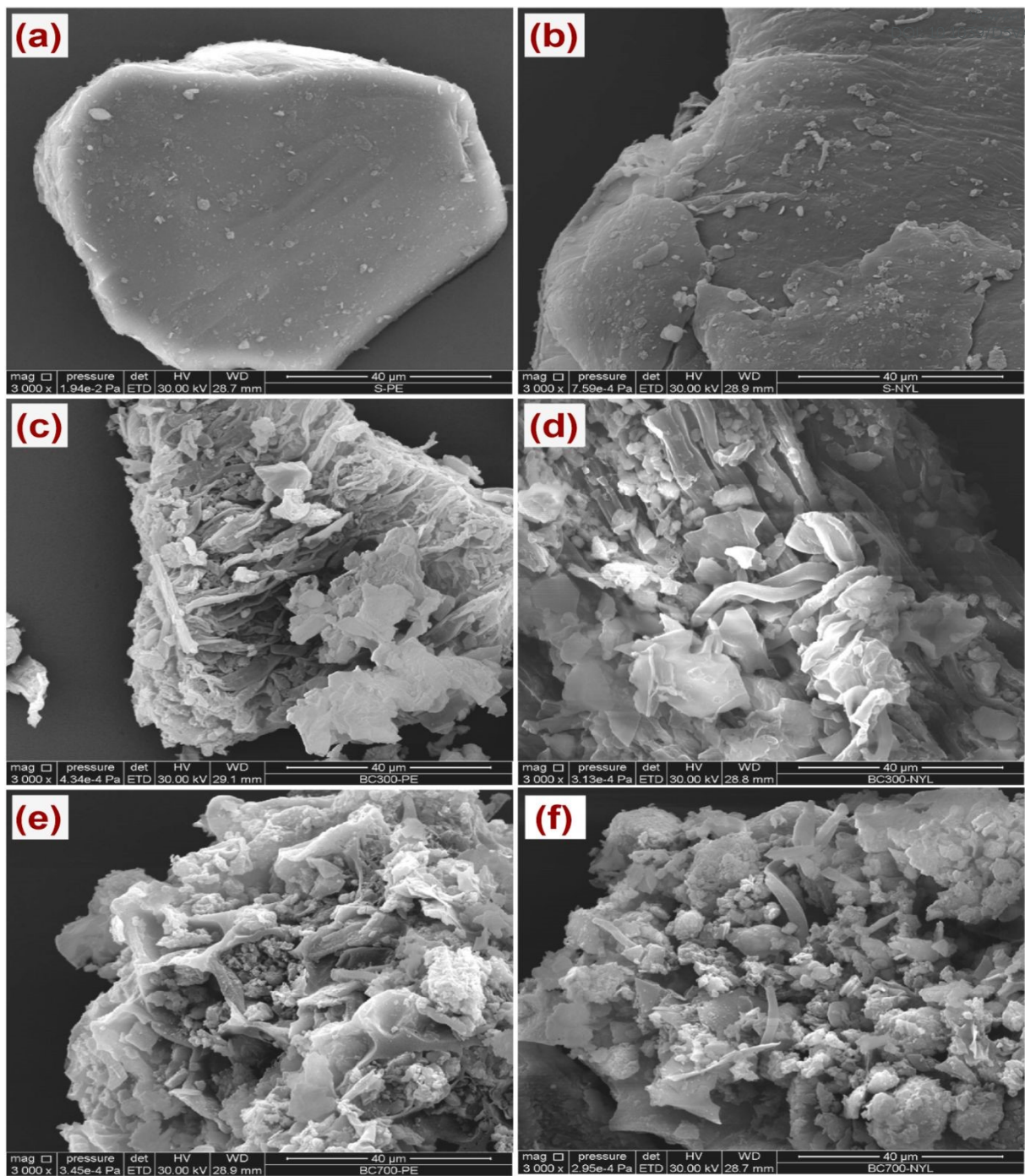
Fig. 7 SEM images showing several removal mechanisms, including adsorption, stuck, and entanglement, of MPs by jujube waste-derived biochar in a simulated trench-based SWMEPMS (adapted from Ahmad et al., with permission from Elsevier, 90 copyright 2023 ). This figure highlights various removal mechanisms by which MPs are retained on sand and biochars derived from jujube waste at two different pyrolysis temperatures: (a) shows PE particles adsorbed onto the surface of sand. We suggest that the smooth surface of the sand may have provided limited attachment points for the PE particles, with retention occurring mainly through weak surface attachment and the ‘stuck’ mechanism, where particles became immobilized within the large inter-particle voids; (b) illustrates how nylon particles were retained on sand, similar to PE, with removal limited to weak attachment on the relatively smooth surface and dominated by the stuck
