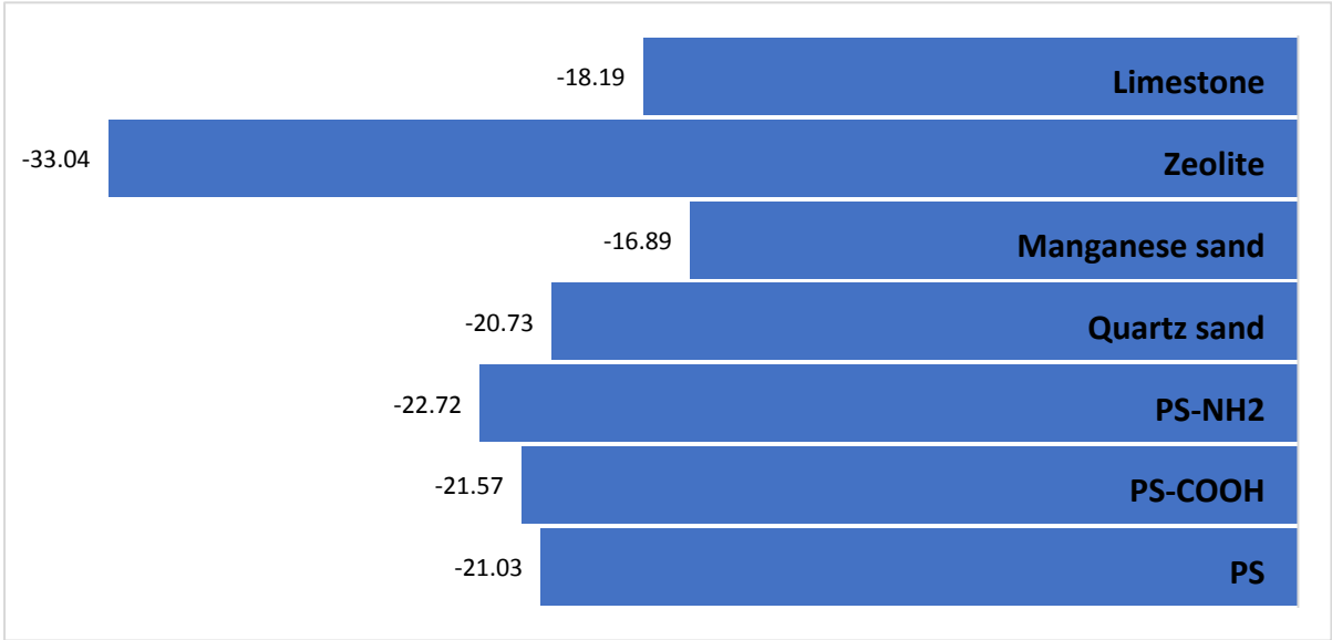
Fig. 5 Zeta potential of NPs and some of the engineered porous media (designed by the authors of this present work using the data reported by Wang et al.) 98 . Deionized water was the background solution used
