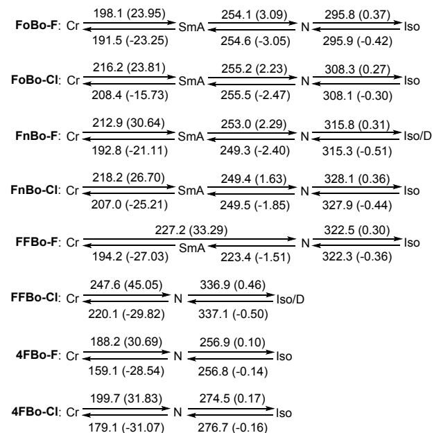
Figure 8. Phase transition temperatures ( ^{\circ}\text{C} ) and enthalpies ( \text{kJ mol}^{-1} ) of derivatives with the inner benzoxazole ( Bo ) partially and fully fluorinated. Values are determined by DSC at 5^{\circ}\text{C/min} under \text{N}_2 for 2 nd -heating and 1 st -cooling runs). Cr = crystalline phase; SmA = smectic A; N = nematic; Iso = isotropic liquid; D = decomposition.
