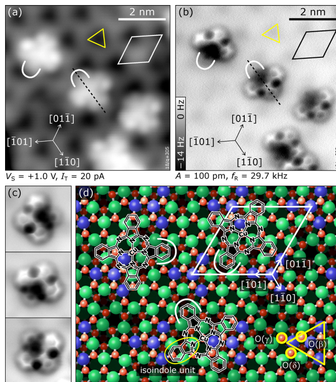
Fig. 2 Isolated CuPc molecules adsorbed on \text{In}_2\text{O}_3(111) . (a) STM image showing CuPc molecules in different rotational orientations. The substrate unit cell is indicated in white. The “dark” region of the unit cell (located at the corners of the unit cell) comprises \text{In}(6c) surface atoms and is highlighted by a yellow triangle. (b) Constant-height AFM image taken at the same spot. (c) Magnification of individual molecules with different orientations measured in constant-height AFM; each image is 2.5 \times 2.5 \text{ nm}^2 in size. (d) Adsorption site of CuPc on \text{In}_2\text{O}_3(111) : molecular structure of CuPc superimposed on the atomic model of the bare \text{In}_2\text{O}_3(111) surface as observed in (a) and (b); the isoindole unit tilted towards the surface, which appears darker in AFM, is marked by a white curve. The adsorption site is described in the text. The yellow triangle marks the arrangement of \text{In}(6c) atoms (blue); \text{In}(5c) are green, \text{O}(4c) are dark red. The three inequivalent \text{O}(3c) atoms (light red) with bonds to the \text{In}(6c) are labelled \beta , \delta , and \gamma ; note that three of each type are symmetrically arranged around the yellow triangle due to the 3-fold symmetry of the surface. All images were acquired at 5 K.
