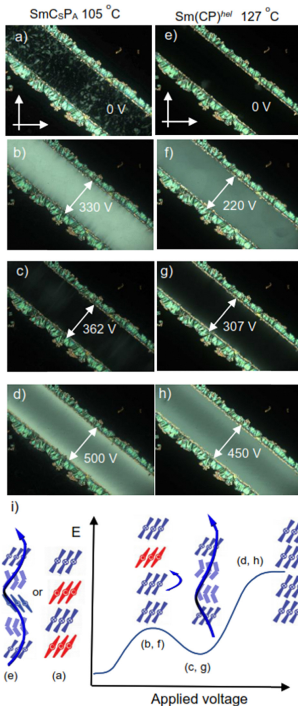
Fig. 11 (a)–(h) POM textures of 1/O12 in an 8 \mu\text{m} homeotropic cell at the indicated temperatures under the given applied in-plane fields; (a)–(d) in the \text{SmC}_\text{sP}_\text{A} temperature range and (e)–(h) in the \text{Sm}(\text{CP})^\text{hel} range; the gap between the electrodes is 180 \mu\text{m} . (i) Shows the schematic energy profile and schematics of the molecular reorganization during the field induced transitions; see Fig. S35 (ESI†) for relaxation experiments and for related data of 1/O10 and 1/O18 , see Fig. S29 and S41 (ESI†).
