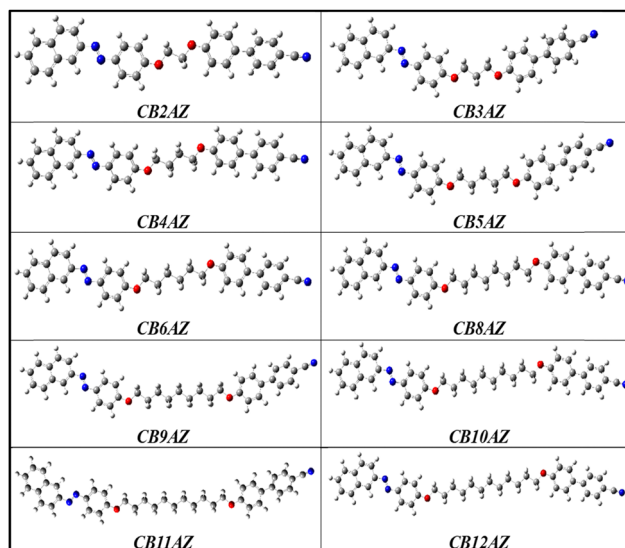
Fig. 6 Optimized molecular structures of series CB n AZ .
