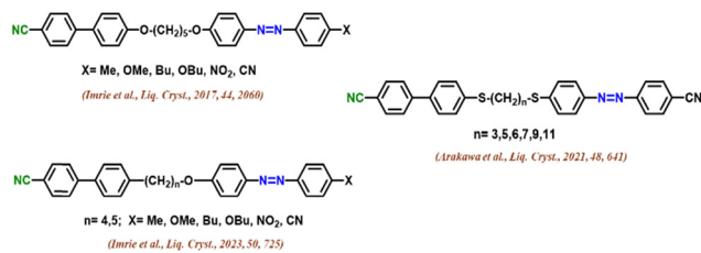
Fig. 1 Asymmetric dimers featuring a combination of cyanobiphenyl and azo moiety.
