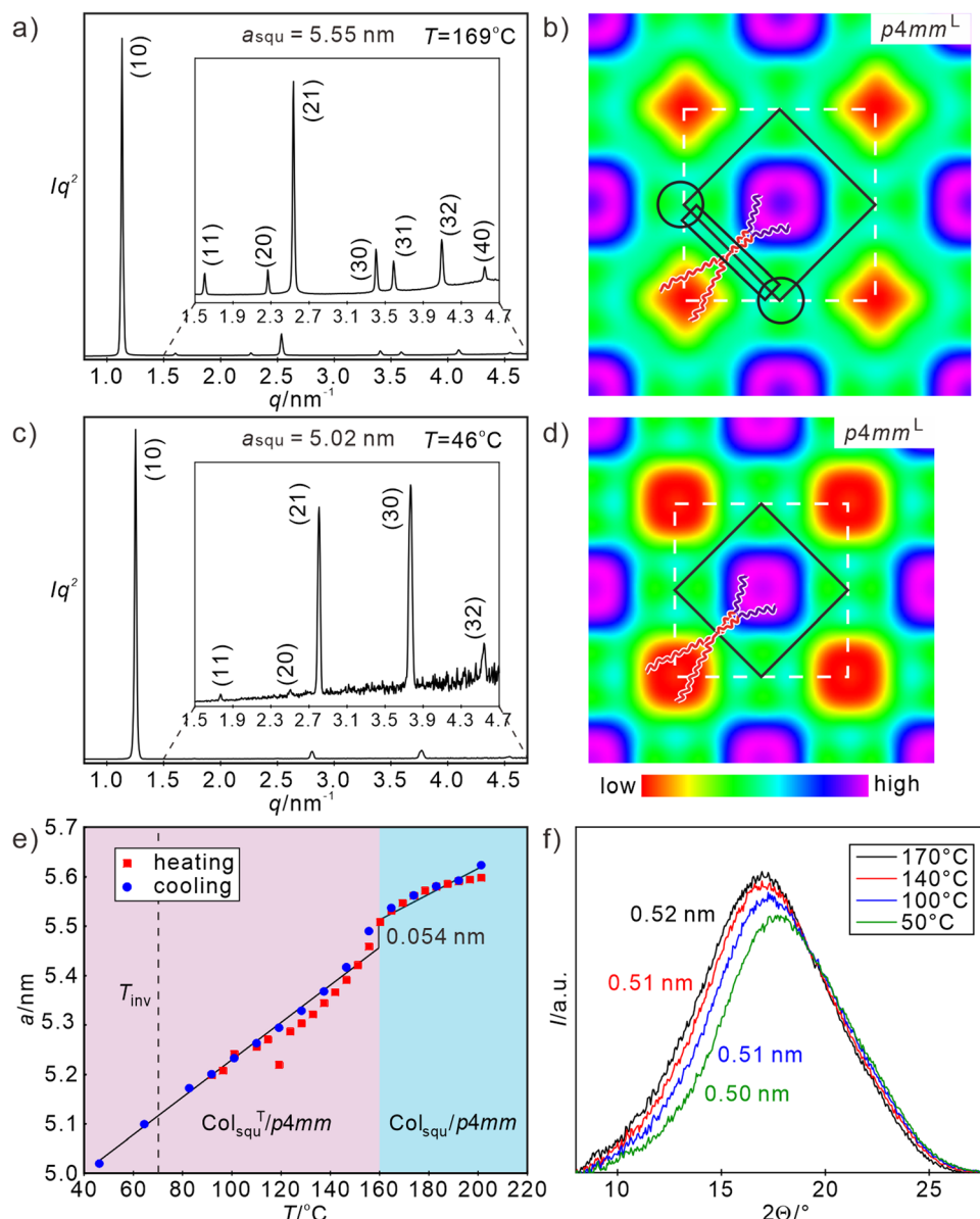
Fig. 3 (a) and (c) SAXS patterns (for numerical data, see Tables S8 and S9, ESI†) and (b) and (d) reconstructed ED maps of the \text{Col}_{\text{sq}}/\text{p4mm}^{\text{L}} phase of H8/16 at 169^\circ\text{C} and 46^\circ\text{C} , respectively (phase choices 00\pi0\pi\pi\pi and 00\pi0\pi\pi ); white dashed lines indicate the unit cell and solid black lines the shape of one honeycomb cell, in (b) a molecular model is drawn, black rectangle indicates the aromatic core and the black circles indicate the glycerol nodes; (e) shows the temperature dependence of a_{\text{sq}} ; (f) shows the diffuse WAXS scatterings at different temperatures (for numerical WAXS data, see Table S1, ESI†). For DSC data and textures, see Fig. S1d and S4 (ESI†).
