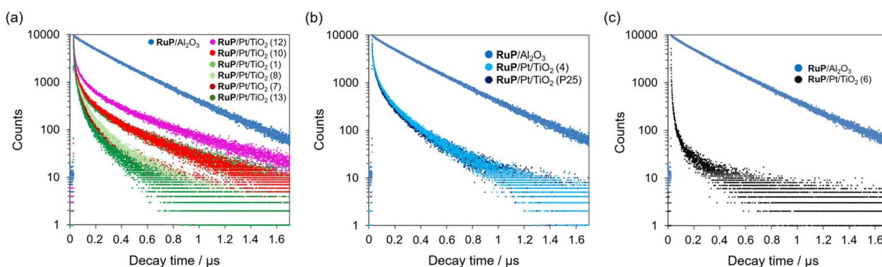
Fig. 4 Emission lifetimes of RuP/Pt/TiO 2 samples with different TiO 2 crystal structures: (a) anatase, (b) mixed phase of anatase and rutile, and (c) rutile. Emission lifetime measurements were performed after introducing 4 mL of an aqueous HCl solution (pH 4) and 3 mg of RuP/Pt/TiO 2 into a dedicated cell, followed by 30 minutes of Ar bubbling to remove dissolved gases, using an excitation wavelength of 451 nm and monitoring the emission at 630 nm.
