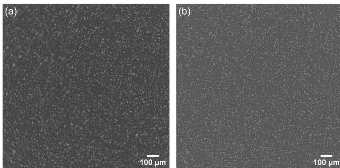
Figure 8. (a) Experimental low-resolution, large field of view (FoV) unseen image of NMC811 cathode. (b) Enhanced resolution, large FoV image generated by using the trained CNN model, improving the level of detail of particle and microstructural characteristics.
