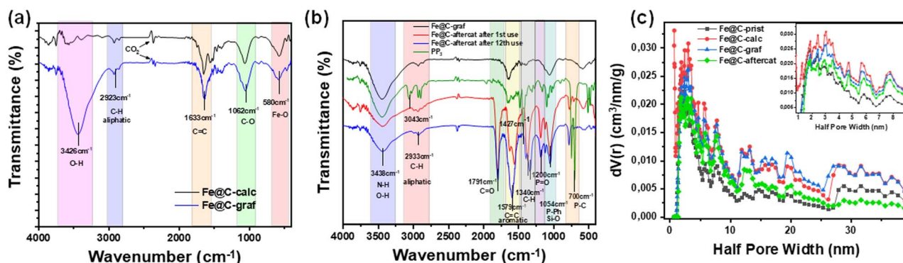
Fig. 5 FT-IR spectra of (a) a comparison of \text{Fe@C} -calc and \text{Fe@C} -graf and (b) comparison among \text{Fe@C} -graf, \text{Fe@C} -aftercat (1st use and 12th use), and \text{PP}_3 . (c) Pore size distribution of all the hybrid materials using the DFT method.
