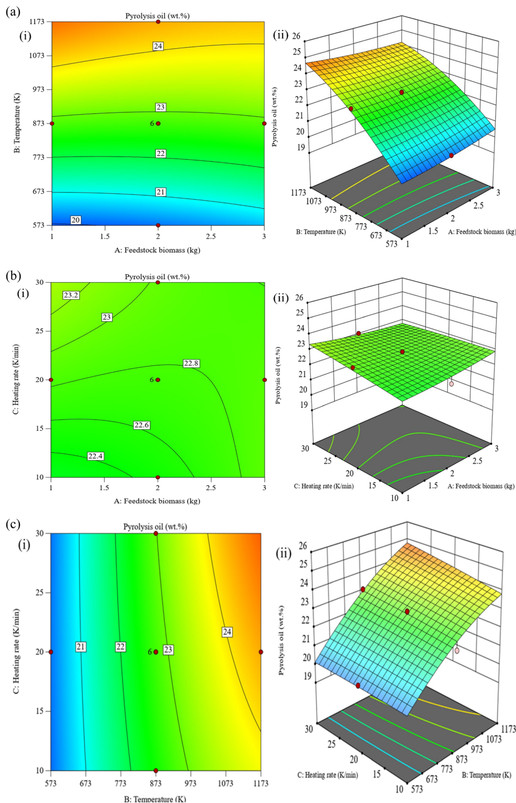
Fig. 7 (a) (i) Two-dimensional contour and (ii) three-dimensional contour plots showing pyrolysis oil yield (wt.%) as a function of feedstock biomass and temperature. (b) (i) Two-dimensional contour and (ii) three-dimensional contour plots showing pyrolysis oil yield (wt.%) as a function of feedstock biomass and heating rate. (c) (i) Two-dimensional contour and (ii) three-dimensional contour plots showing pyrolysis oil yield (wt.%) as a function of heating rate and temperature.
