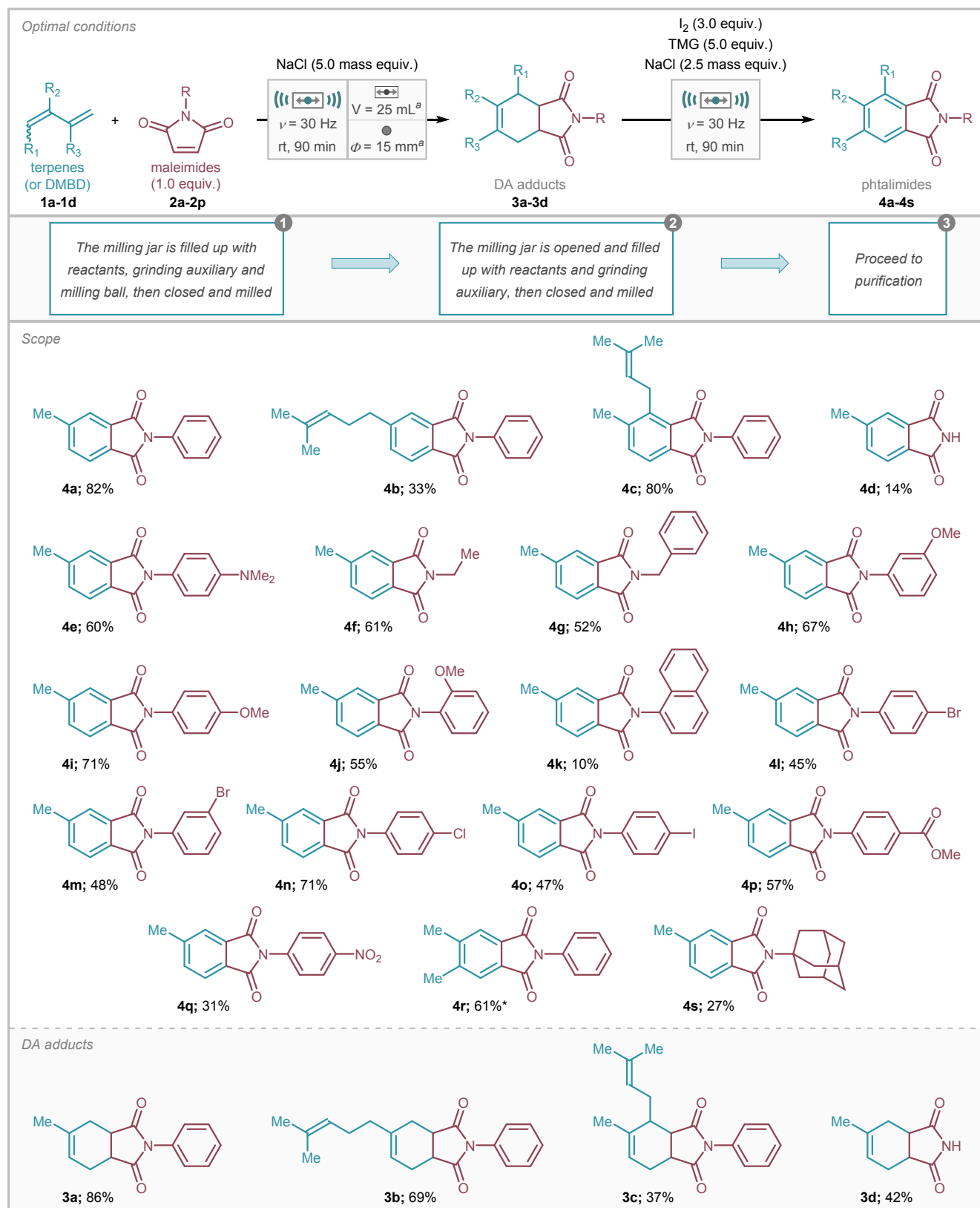
Scheme 1 Optimized one-pot tandem protocol for the production of phthalimides 4a–4s . a Stainless steel materials. *Non-terpene DMBD used.
