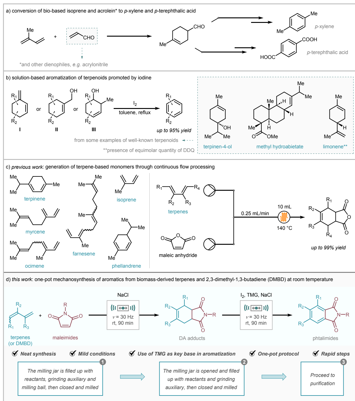
Figure 1 Terpenes and terpenoids as powerful starting materials for chemical valorization towards aromatics.
