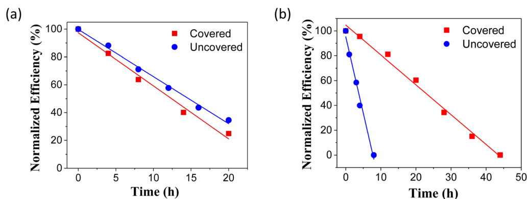
Fig. 3 Normalized average efficiency of 12 mixed (a) and pure (b) perovskite solar cells versus light exposure time. Non coated samples are shown as blue circles, white coated samples are shown as red squares.
