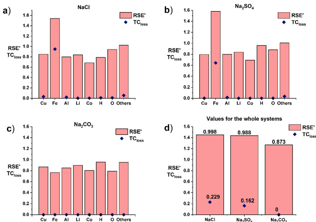
Fig. 2 \text{TC}_{\text{loss}} and \text{RSE}' of different discharging systems: (a) NaCl, (b) \text{Na}_2\text{SO}_4 , (c) \text{Na}_2\text{CO}_3 , and (d) the whole systems.
