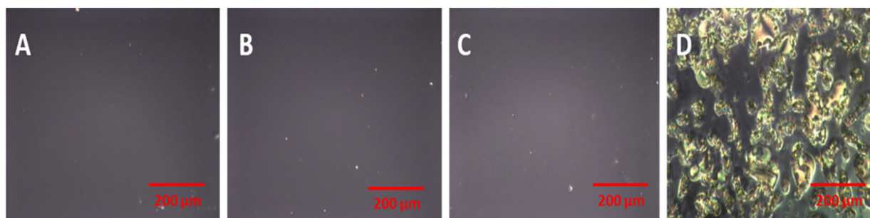
Fig. 6 Optical images (under cross polarizer) of LC cells in the presence of different concentrations of folate@GNP (A) 1 μg mL -1 , (B) 2 μg mL -1 , (C) 5 μg mL -1 and (D) 10 μg mL -1 .
