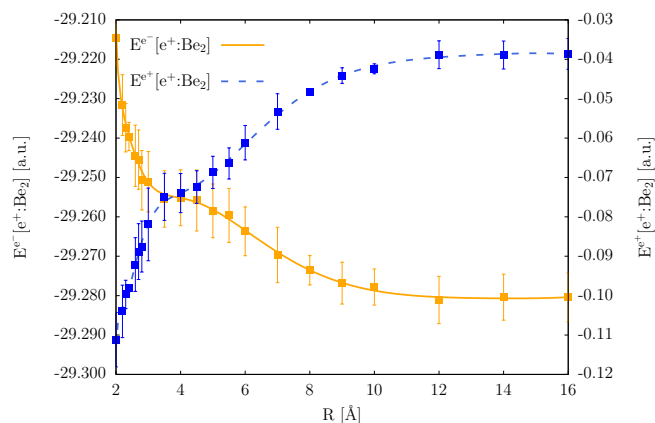
Fig. 3 Electronic energy ( E^{\text{e}^-}[\text{e}^+:\text{Be}_2] ), and positronic energy ( E^{\text{e}^+}[\text{e}^+:\text{Be}_2] ) contributions. Error bars represent one standard error on the mean.
