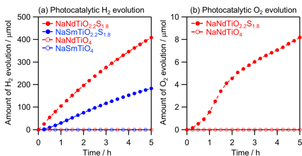
Fig. 8 Time courses of photocatalytic (a) \text{H}_2 and (b) \text{O}_2 evolution on \text{NaMTiO}_4 ( M = \text{Nd}, \text{Sm} ) and \text{NaMTiO}_{2.2}\text{S}_{1.8} from water with an electron donor ( \text{S}^{2-} , \text{SO}_3^{2-} ) and acceptor ( \text{Ag}^+ ), respectively, under visible light ( 400 < \lambda < 800 \text{ nm} ).
