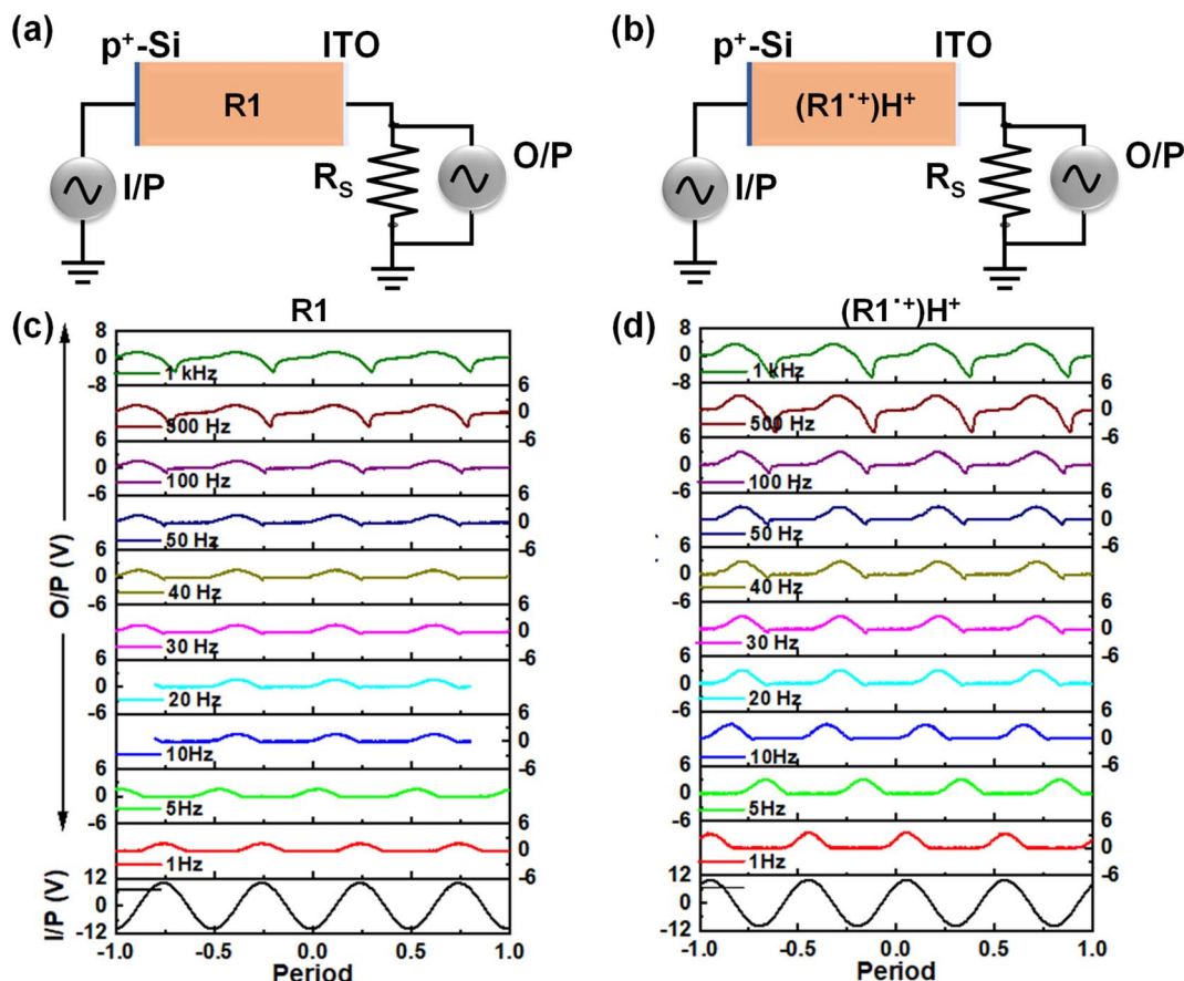
Fig. 4 Investigation of alternating current to direct current conversion efficiency. (a) A measurement setup for AC to DC signal conversion for R1 and (b) (R 1 H + )H + . (c) Conversion of AC to DC signals of p + -Si/ R1 58 nm /ITO and (d) p + -Si/ (R 1 H + )H + 58 nm /ITO after 60 s of exposure. The data were collected at different frequencies (minimum 1 Hz and maximum 1 kHz).
