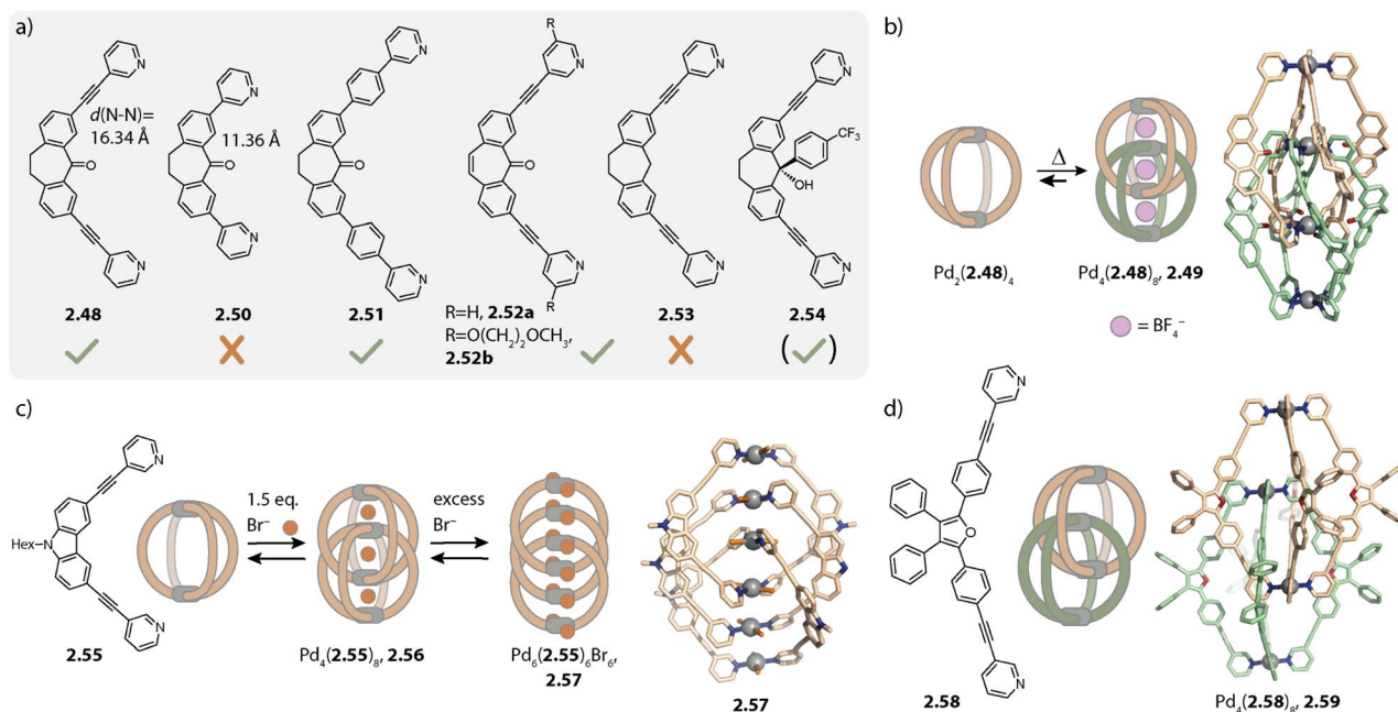
Fig. 9 Interlocked double cages \text{Pd}_4\text{L}_8 . (a) Structures of suberone-based ligands 2.48 – 2.54 (check mark: forms a double cage; cross: does not form a double cage). (b) Self-assembly of monomeric cage \text{Pd}_2(\text{2.48a})_4 as a kinetic product and double cage 2.49a as the thermodynamic product. (c) Halide induced formation of double cage 2.56 and ligand release upon addition of excess halides to form triple catenated 2.57 in the solid state. (d) Triply interlocked double cage 2.59 with furane based ligand 2.58 .
