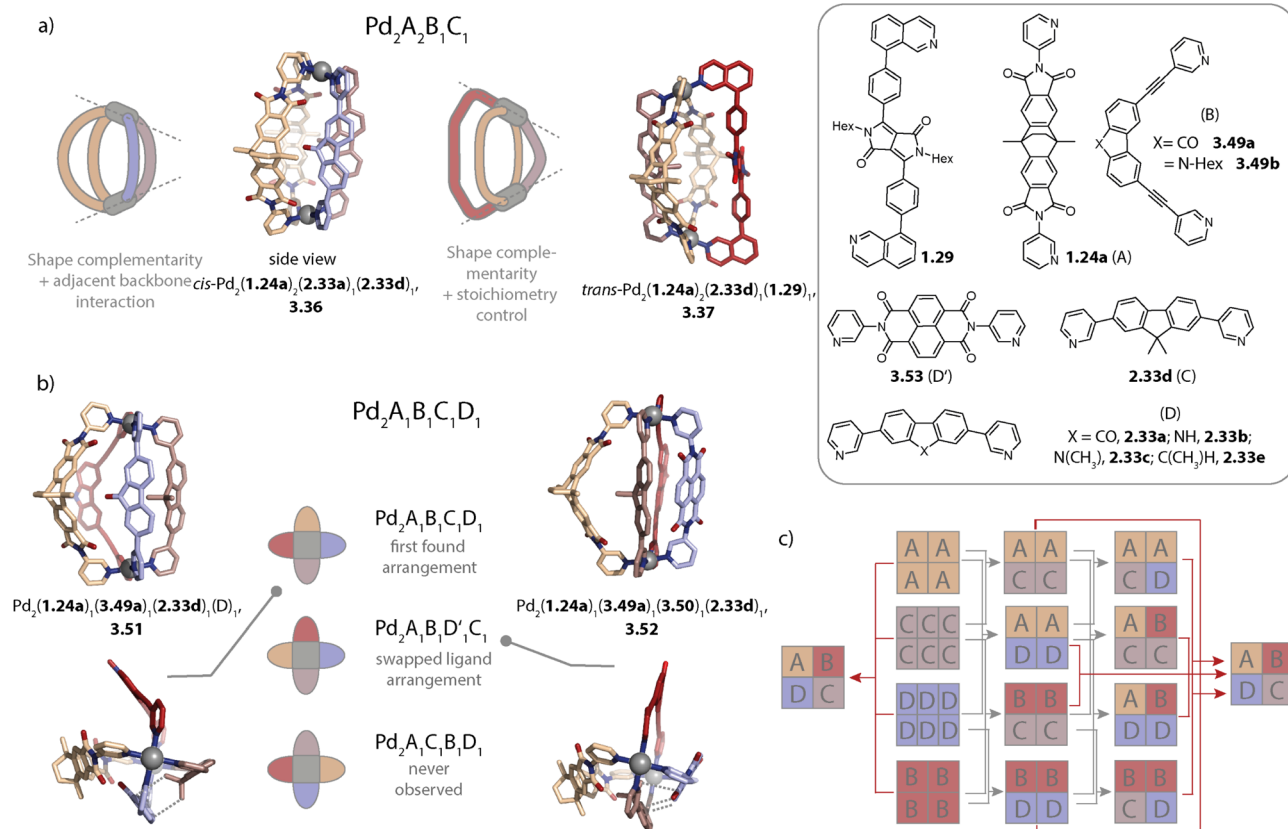
Fig. 16 Integrative self-sorting to \text{Pd}_2\text{A}_2\text{B}_1\text{C}_1 -type and \text{Pd}_2\text{A}_1\text{B}_1\text{C}_1\text{D}_1 -type cages under thermodynamic control. (a) Structures of \text{cis-Pd}_2\text{A}_2\text{B}_1\text{C}_1 -type cage 3.36 and \text{trans-Pd}_2\text{A}_2\text{B}_1\text{C}_1 -type cage 3.37 obtained by combining the SCA approach with the ABI approach or stoichiometry control, respectively. (b) Illustration of the three possible ligand arrangements in \text{Pd}_2\text{A}_1\text{B}_1\text{C}_1\text{D}_1 -type cages and X-ray structures of realized pseudo-isomers 3.51 and 3.52 , selectively formed as one of 55 homo- and heteroleptic dinuclear cages possible in principle. (c) All possible pathways for the synthesis of the \text{Pd}_2\text{A}_1\text{B}_1\text{C}_1\text{D}_1 -type cage via cage-to-cage transformations.
