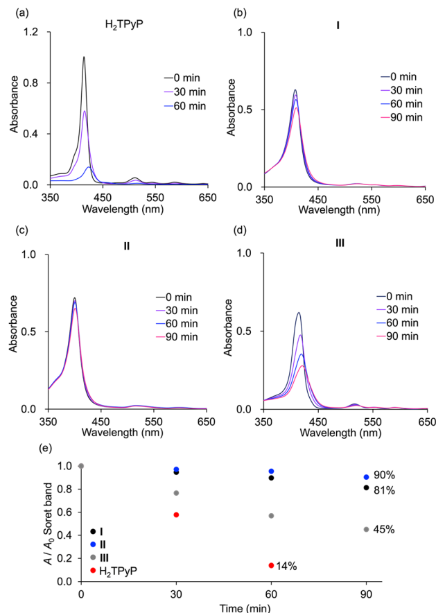
Fig. 7 Time-dependent absorption spectra of (a) \text{H}_2\text{TPyP} and (b) hybrid I , (c) hybrid II , and (d) hybrid III in acetonitrile/dichloromethane (1/1, v/v) upon photoirradiation ( \lambda > 350 \text{ nm} ) in air. (e) Changes in the A/A_0 values of the Soret band of hybrids I , II , and III and \text{H}_2\text{TPyP} ( A : Soret band intensity; A_0 : initial Soret band intensity).
