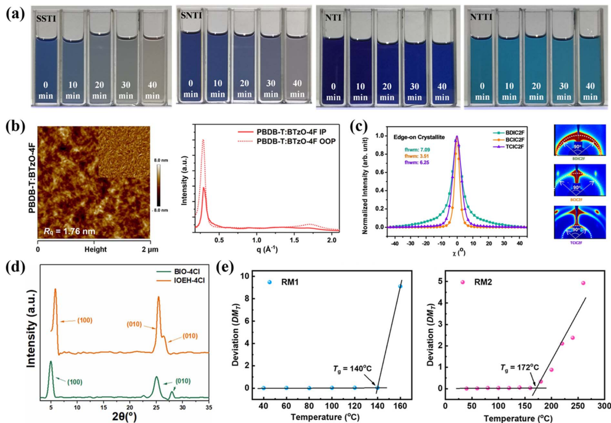
Fig. 6 (a) Optical images of D:A solutions (PCE10:SSTI vs. PM6:NTI vs. PBDB-T:NTI/NTTI) under AM1.5G light illumination. Reproduced with permission. 68 Copyright 2020, John Wiley and Sons. (b) AFM morphology and GIWAXS line profiles (IP/OOP) of PBDB-T:BTzO-4F blend films. Reproduced with permission. 69 Copyright 2020, Springer Nature. (c) Azimuthal scans and corresponding 2D GIWAXS patterns of three NFRA. Reproduced with permission. 73 Copyright 2021, John Wiley and Sons. (d) XRD patterns of the BIO-4Cl and IOEH-4Cl pristine solid powders. Reproduced with permission. 77 Copyright 2023, Elsevier. (e) DMT evolution with annealing temperature for RM1 and RM2 thin films. Reproduced with permission. 79 Copyright 2024, American Chemical Society.
