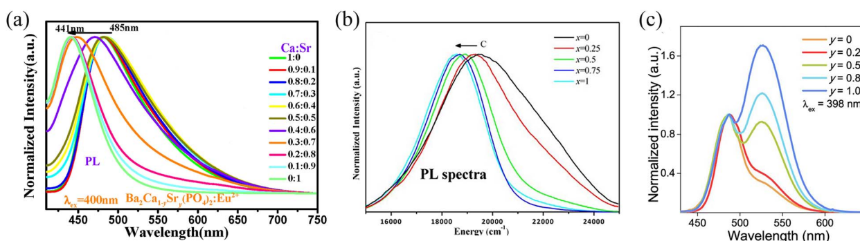
Fig. 4 (a) Normalized PL spectra of \text{Ba}_2\text{Ca}_{1-x}\text{Sr}_y(\text{PO}_4)_2:\text{Eu}^{2+} . Reproduced with permission from ref. 113. Copyright 2020, Elsevier. (b) PL spectra of the phosphors \text{Ca}_{1.98}(\text{Al}_{1-x}\text{Mg}_x)(\text{Al}_{1-x}\text{Si}_{1+x})\text{O}_7:0.02\text{Eu}^{2+} ( x = 0, 0.25, 0.5, 0.75 , and 1) as a function of x . Reproduced with permission from ref. 116. Copyright 2015, ACS. (c) Normalized PL spectra of \text{CsKNa}_{1.98-y}\text{Li}_y(\text{Li}_3\text{SiO}_4)_4:0.02\text{Eu}^{2+} ( 0 \leq y \leq 1 ). Reproduced with permission from ref. 76. Copyright 2019, ACS.
