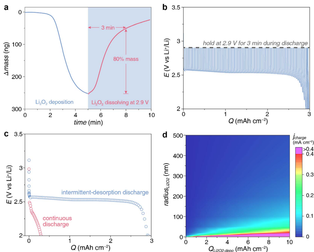
Fig. 5 The consequence of slow dissolution process on discharging and charging process. (a) The dissolution of the Li 2 O 2 deposited on the electrode (Au–O 2- ) surface when applying a potential of 2.9 V. (b) Load curve for discharging a Li–O 2 cell with intermittent-desorption discharge mode. After every 10 minutes of galvanostatic discharge, the cell is held at 2.9 V for 3 minutes. Current density: 0.22 mA cm -2 . (c) Comparison between intermittent-desorption discharge and continuous galvanostatic discharge at the same current density of 0.22 mA cm -2 . (d) The estimate of the maximum charging current under the given discharge capacity and product particle size.
