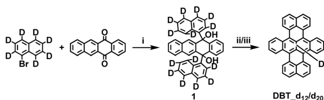
Scheme 1 Synthetic route to DBT_d 12 and DBT_d 20 . Reagents and conditions: (i) n -BuLi, 5,12-naphthacenequinone, THF, -78 °C, 60%; (ii) AlCl 3 , NaCl, 140 °C, 10 min, 20% for DBT_d 12 ; (iii) AlCl 3 , chlorobenzene-d 5 , 100 °C, 1 h, 50% for DBT_d 20 .
