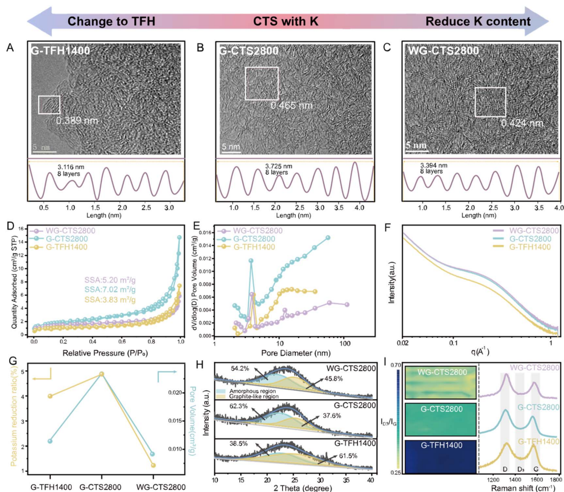
Fig. 1 Structural characterization of G-TFH1400, G-CTS2800 and WG-CTS2800. (A–C) HRTEM images. (D) \text{N}_2 adsorption/desorption isotherms. (E) Pore size distribution according to the BJH method and (F) SAXS patterns of various HCs. (G) A graph illustrating the pore-forming effect induced by potassium: the fraction of potassium reduction and the pore volume in various HCs. (H) The broad XRD peak of (002) is divided into two regions: an amorphous region and a graphite-like region. (I) The mapping of Raman spectra quantified by the intensity ratio of the \text{D}_3 band to the G band ( I_{\text{D}_3}/I_{\text{G}} ).
