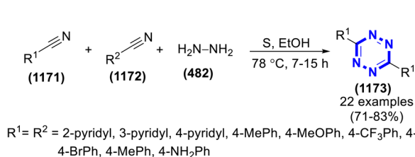
Scheme 325 Synthesis of 1,2,4,5-tetrazines catalyzed by elemental sulfur.
