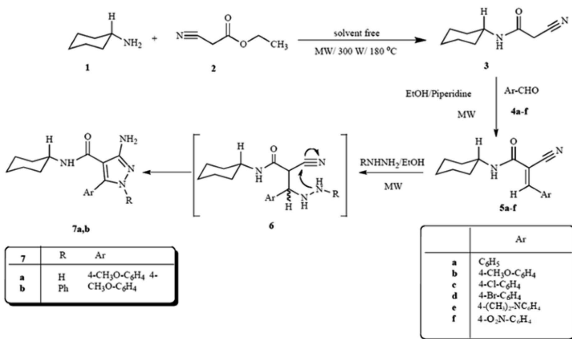
Scheme 14 Synthesis of 2-cyano- N -cyclohexylacetamide ( 3 ), followed by its reaction with aromatic aldehyde derivatives and the subsequent reaction of acrylamide derivatives with hydrazine derivatives. 81
