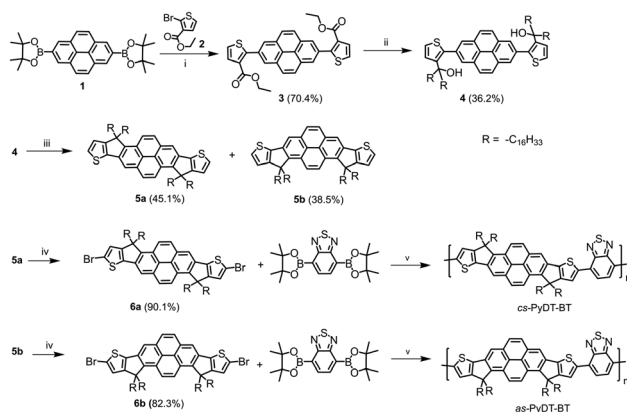
Scheme 1 Synthetic routes of the polymer cs-PyDT-BT and as-PyDT-BT . Regents and conditions: (i) \text{Pd}(\text{PPh}_3)_4 , \text{K}_2\text{CO}_3 , toluene/water, 110 °C; (ii) \text{C}_{16}\text{H}_{33}\text{MgBr} , THF, reflux; (iii) Amberlyst 15 (H), toluene, 110 °C; (iv) NBS, \text{CHCl}_3 , –20 °C; (v) Buchwald-G3-XPhos, \text{K}_2\text{CO}_3 , toluene/water, 90 °C.
