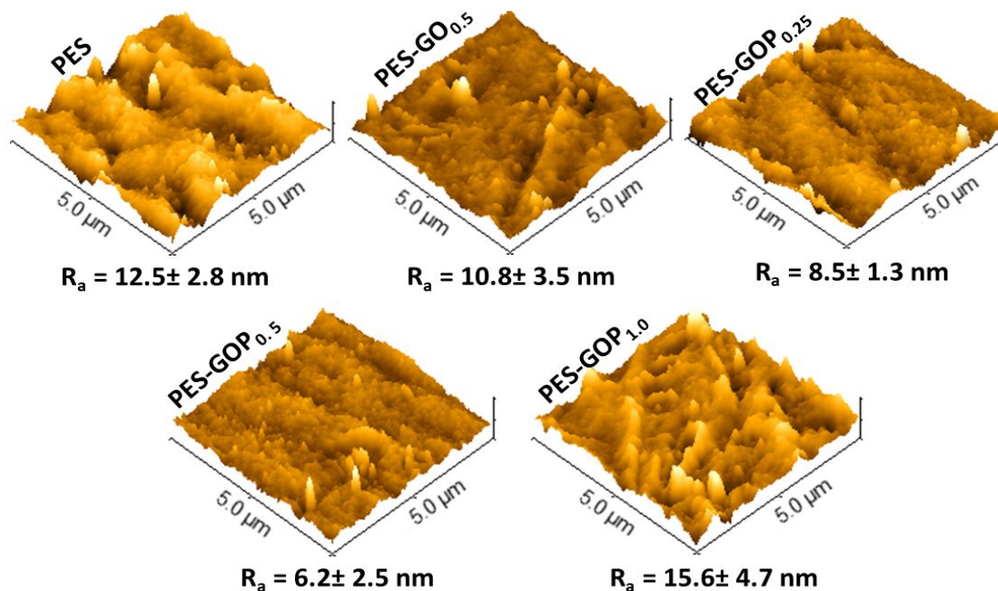
Figure 7. Three-dimensional AFM images of PES substrates modified with GO and GO-g-PDMA nanofillers, showing variations in surface roughness.
