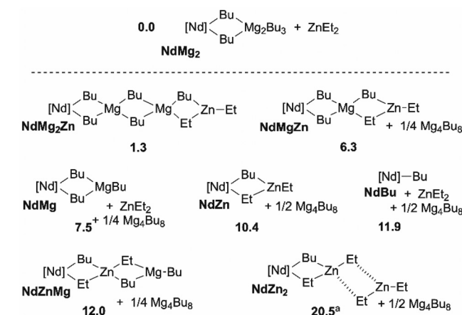
Scheme 3 Speciation of the alkylated species yielded from [\text{Nd}]-^n\text{Bu} , \text{Mg}_4^{\text{n}}\text{Bu}_8 and \text{ZnEt}_2 . Only the most stable species are shown, the fully detailed speciation is provided in ESI.† \Delta G in kcal mol -1 . a In NdZn 2 , interaction between the \text{ZnEt}_2 fragments is weak, the endergonicity results from the entropy cost of the association of free and separated \text{ZnEt}_2 . Gaussian 09, B3PW91/D3BJ(SP), SMD(TolH), 298 K, 1 atm.
