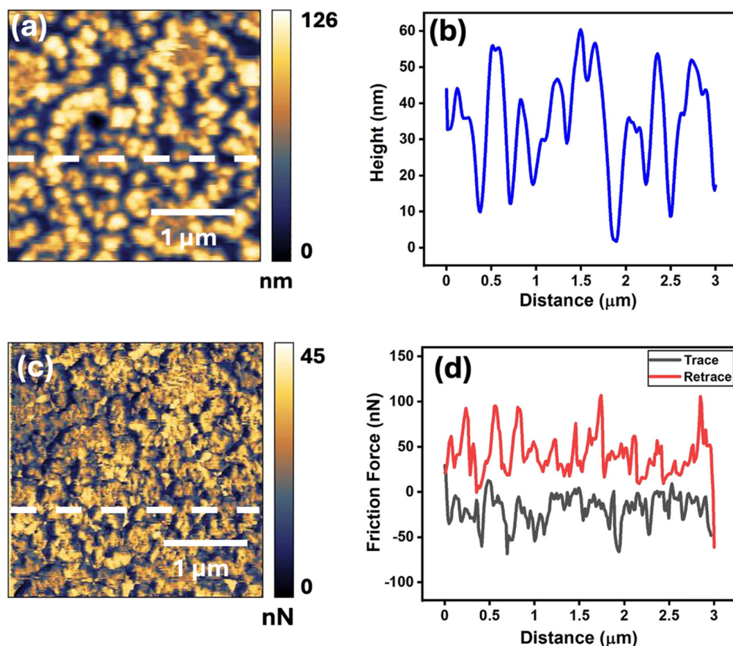
Fig. 3 LFM performed on the pure PANI thin film applying a normal load of 10 nN using a sharp AFM tip: (a) topography of the pure PANI thin film and (b) the profile of the white line from image a; corresponding (c) lateral force map (captured during the forward movement of the cantilever/trace motion) and (d) the profile of the white line or the friction loop from image c.
