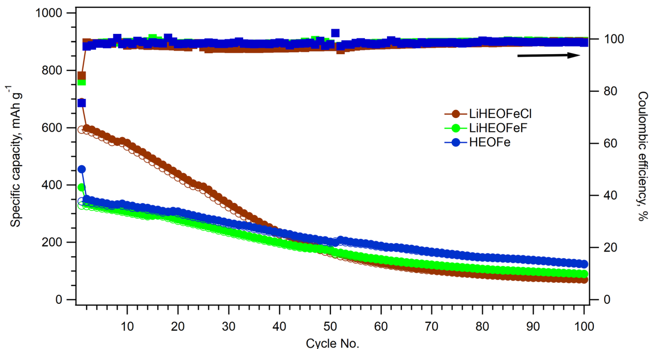
Fig. 7 Galvanostatic chronopotentiometry at 1C rate for HEOFe (blue circles), LiHFeOFeCl (brown circles), and LiHFeOFeF (green circles). The charge capacity within charging is marked with full circles and the charging capacity within discharging with empty circles. The corresponding coulombic efficiencies for HEOFe, LiHFeOFeCl, and LiHFeOFeF are depicted by squares of the same color coding.
