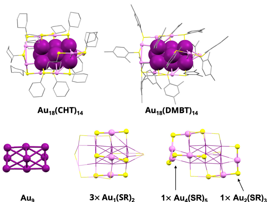
Scheme 1 Atomic structures of Au 18 (CHT) 14 and Au 18 (DMBT) 14 nanoclusters. Color code: purple, pink: gold; yellow: sulfur; gray: carbon. Hydrogen atoms are omitted for clarity.
