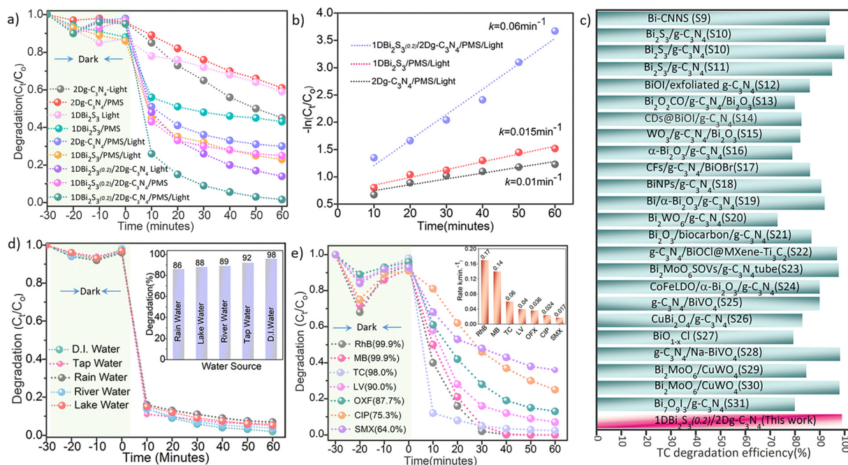
Fig. 4 (a) TC degradation performance of 1D Bi 2 S 3 , 2D g-C 3 N 4 and 1D Bi 2 S 3 (0.2)/2D g-C 3 N 4 under different conditions (with/without PMS/light). (b) Kinetics curves of the TC degradation of photocatalyst/PMS/light systems. (c) Comparison of TC degradation efficiency of this work with some literature reported Bi and g-C 3 N 4 heterostructures. (d) TC degradation efficiency of the 1D Bi 2 S 3 (0.2)/2D g-C 3 N 4 /PMS/light system in various water matrices. (e) General applicability of the 1D Bi 2 S 3 (0.2)/2D g-C 3 N 4 /PMS/light system towards various antibiotics and dye degradation (inset: rate constant ( k ) values). (Reaction condition: [TC] = 20 mg L -1 , [catalyst] = 30 mg, PMS = 2 mM and pH = 7).
