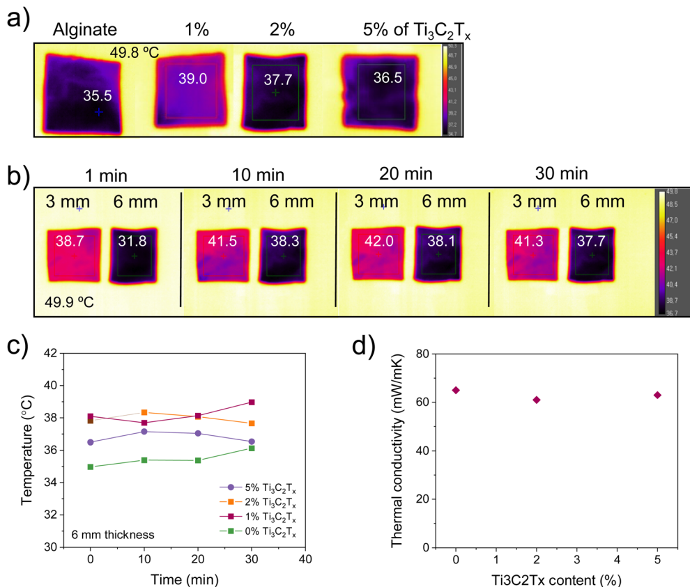
Fig. 4 Thermal insulation behavior of foams. Thermographic camera images of 6 mm thick alginate and Ti 3 C 2 T x -alginate foams taken after 30 min on a 50 °C-hot plate (a) and of 2%Ti 3 C 2 T x -alginate foams with different thicknesses (3 and 6 mm) at different times (b), respectively. Evolution of the surface temperature of 6 mm foams with varying Ti 3 C 2 T x content (c). Thermal conductivity of Ti 3 C 2 T x -alginate foams (d) including error bars of 1 and 0 mW k -1 m -1 .
