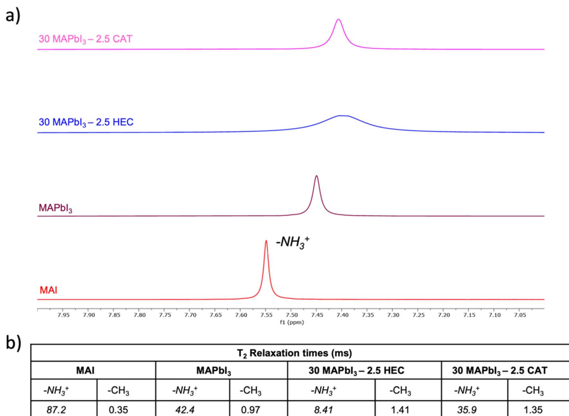
Fig. 2 Nuclear magnetic resonance analysis. (a) 1 H-NMR spectra of 30 MAPbI 3 - 2.5 CAT, 30 MAPbI 3 - 2.5 HEC, reference MAPbI 3 and MAI samples in DMSO-d 6 focused on -\text{NH}_3^+ shift. (b) -\text{NH}_3^+ and -\text{CH}_3 T_2 relaxation times of 30 MAPbI 3 - 2.5 CAT, 30 MAPbI 3 - 2.5 HEC, MAPbI 3 and MAI samples in DMSO-d 6 measured by Carr–Purcell–Meiboom–Gill (CPMG) sequence.
