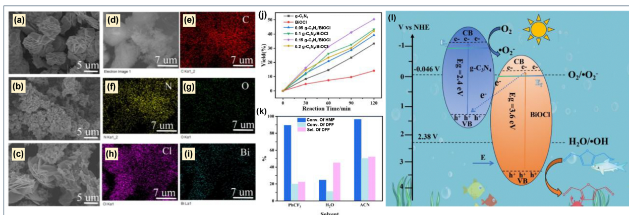
Fig. 58 SEM image of (a) BiOCl, (b) g-C_3N_4 , (c) g-C_3N_4 /BiOCl, (d)–(i) EDS mapping of g-C_3N_4 /BiOCl, (j) photocatalytic activity of various synthesized catalysts, (k) effect of solvents in the photocatalytic oxidation reaction over g-C_3N_4 /BiOCl, (l) Z-scheme charge carrier separation mechanism for photocatalytic oxidation reaction. Reproduced with permission. 283 Copyright 2024, Elsevier.
