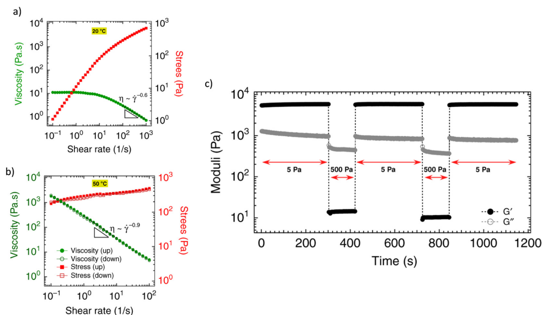
Fig. 8 Yield stress with total recovery: (a) pseudoplasticity of a thermogelling nanoemulsion below 20\text{ }^{\circ}\text{C} (sol state), (b) time-independent plastic behaviour ( n \sim 0 ) (gel state) above 50\text{ }^{\circ}\text{C} , and, (c) total recovery of the moduli. Data reprinted with permission from ref. 114. Copyright © 2019 Nature Comm.
