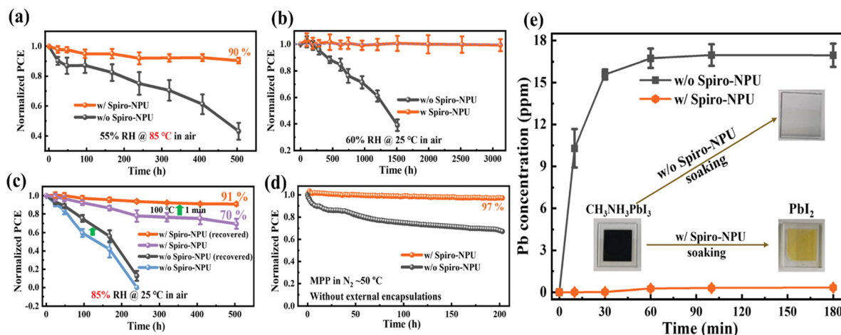
Fig. 14 (a)–(c) Comparative stability analysis of PSCs with and without Spiro-NPU internal encapsulation under varied moisture and temperature conditions. (d) Maximum power point (MPP) tracking of PSCs under AM1.5G, 100 \text{ mW cm}^{-2} solar spectrum conducted in a glovebox. (e) Water-soaking test for MAPbI 3 with and without Spiro-NPU, displaying lead leakage measurements. Reproduced with permission from ref. 211.
